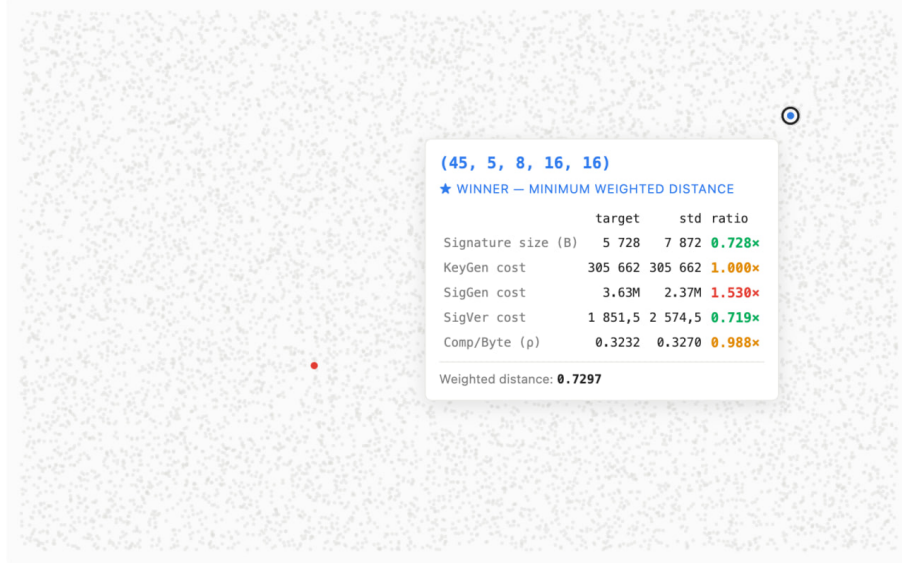
Figure 7: Visualization of the search process under size- and verification-weighted priorities (Case 2).
