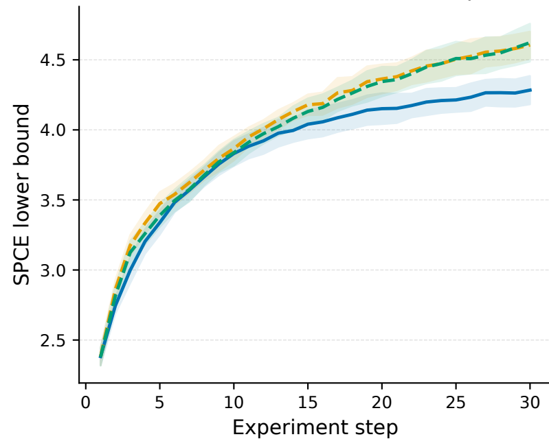
(a) SPCE lower bound vs. step
