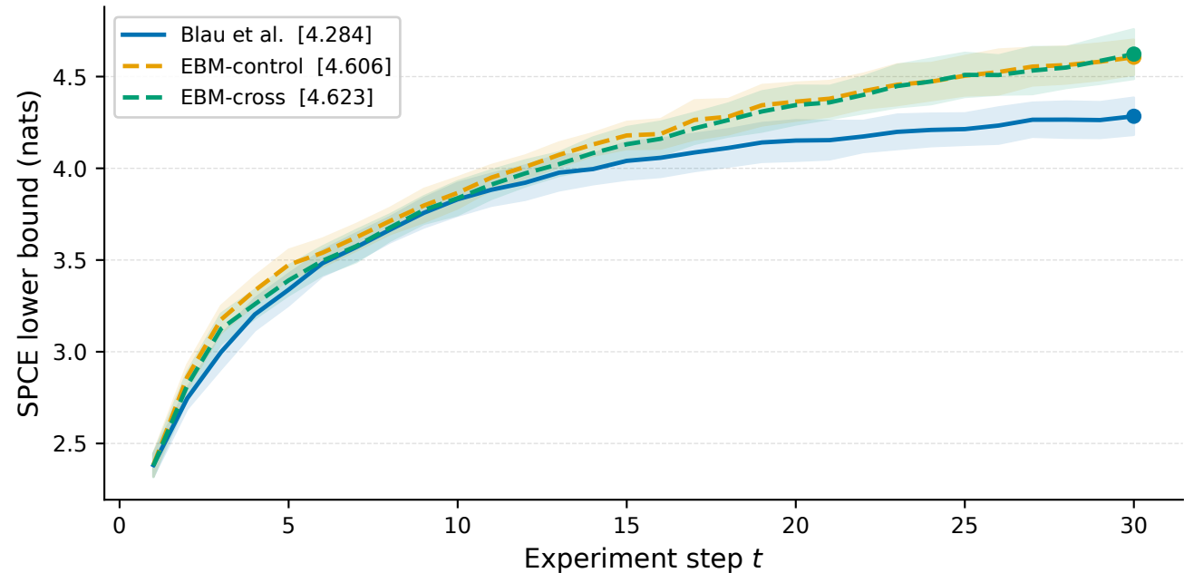
SPCE lower bound vs. experiment step
