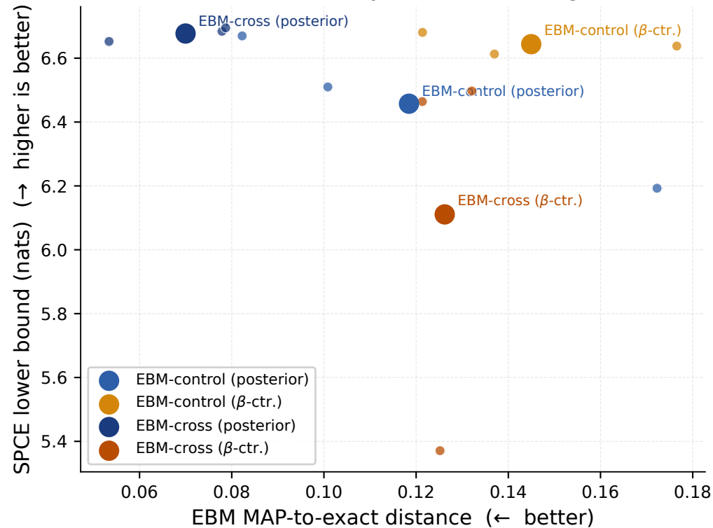
EBM MAP accuracy vs. information gain
