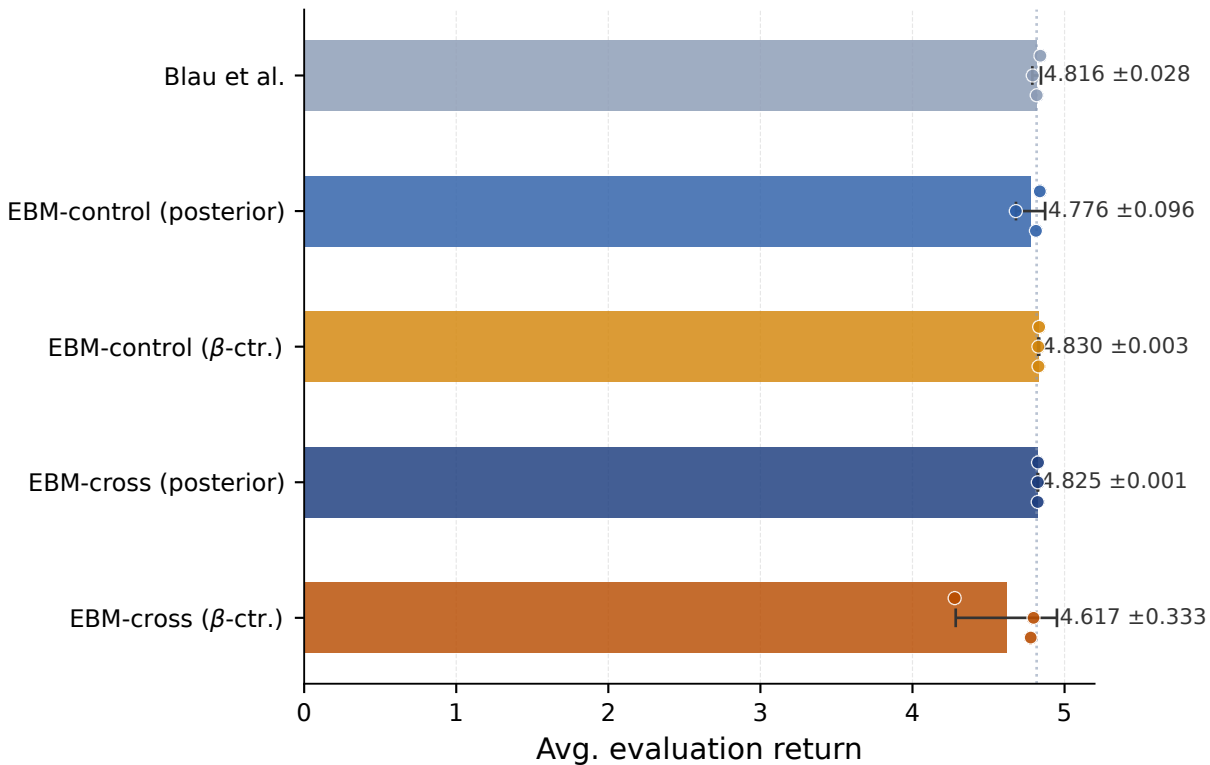
Evaluation return (mean \pm 95 % CI)
