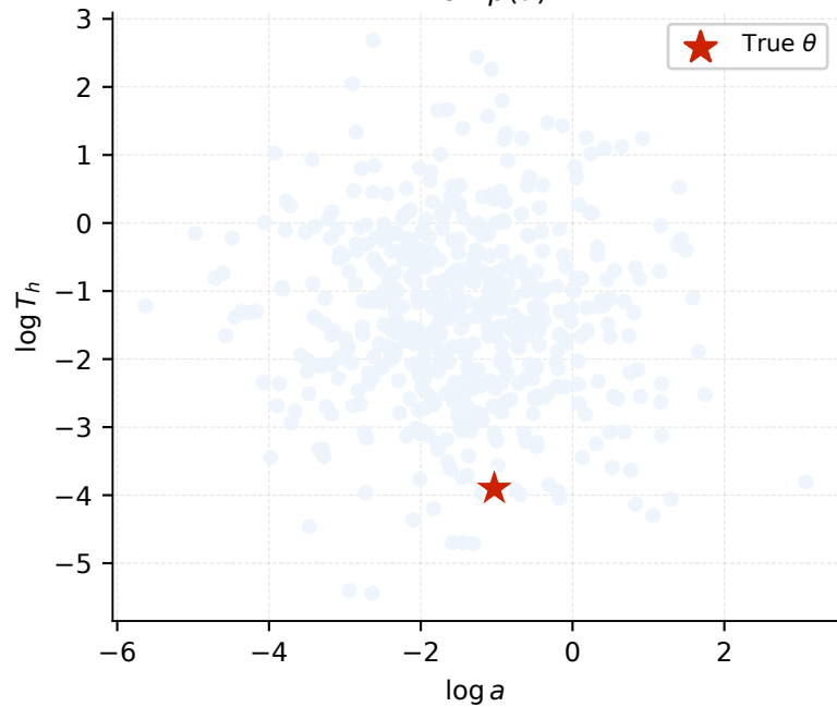
Prior p(\theta)
