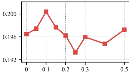
NDCG@10
