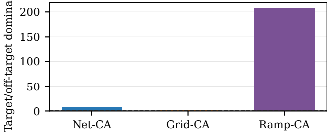
Target concepts dominate individual off-target changes
