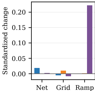
Concept selectivity
