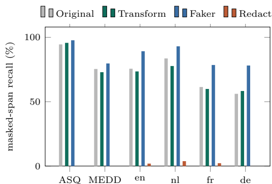
Figure 3: What structure preservation buys (C1/C2; Presidio masked-span recall). Transform tracks the original, the open Faker baseline is at least as high, and redaction collapses to \approx 0 . The gap between the Transform/Faker bars and the Redact bar is the detectability that structure preservation retains.
