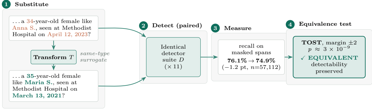
Figure 1: The paired evaluation protocol, with a worked example. (1) The transform replaces each PHI value with a same-type surrogate ( original → surrogate ), leaving everything else byte-identical. (2) The identical 11-detector suite scores both the original d and the transformed d' , so any per-span change is attributable to the substitution alone. (3) Utility is measured only on the spans the transform masks (overlap match), decoupling it from coverage. (4) The paired recall difference is assessed with an equivalence test (TOST, margin \pm 2 pts) rather than a significance test—which the large sample would make trivially “significant” (§4). Result: the change is statistically equivalent to zero.
