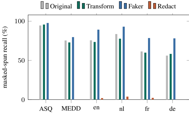
Figure 3: What structure preservation buys, shown for Presidio (which has full original/transform/Faker/redact columns). Transform tracks the original, the open Faker baseline is at least as high, and redaction collapses to \approx 0 . The gap between the Transform/Faker bars and the Redact bar is the detectability structure preservation retains; the family-dependent floor and open-surrogate retention across four detectors are in Tables 4–5.
