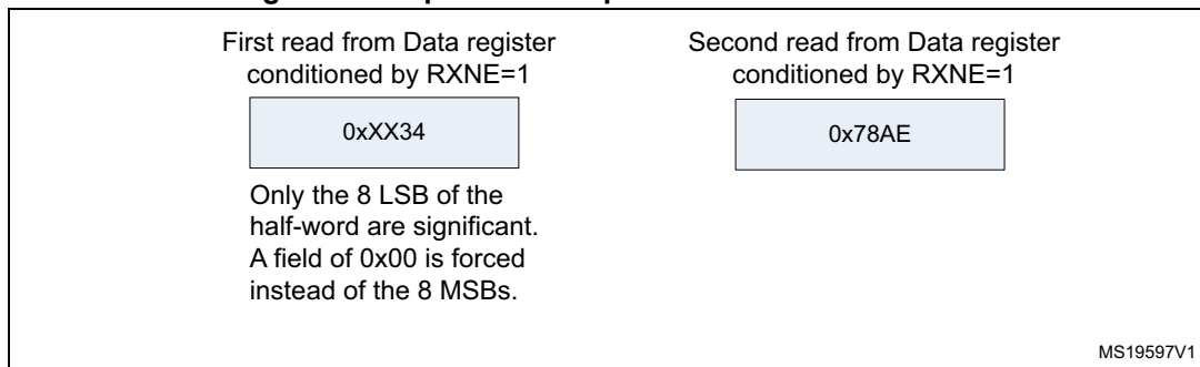
Figure 276. Operations required to receive 0x3478AE
