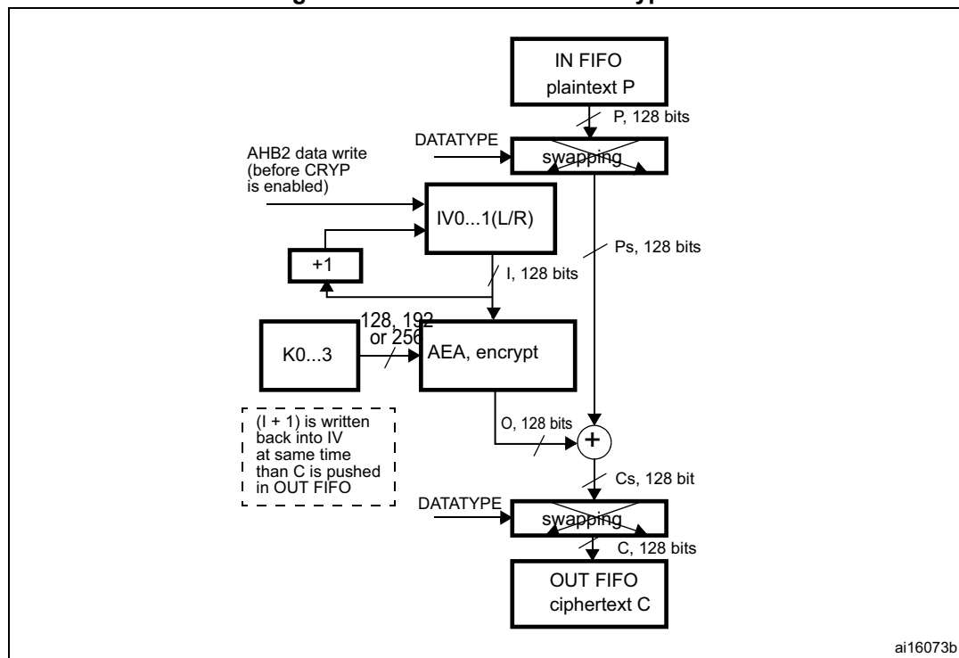
Figure 226. AES-CTR mode encryption
