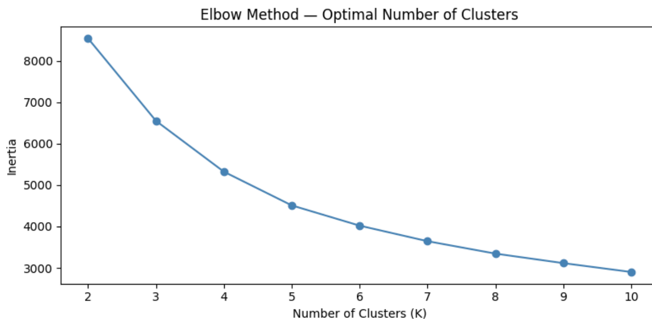
Figure 3: Elbow method plot showing inertia vs. number of clusters K.
