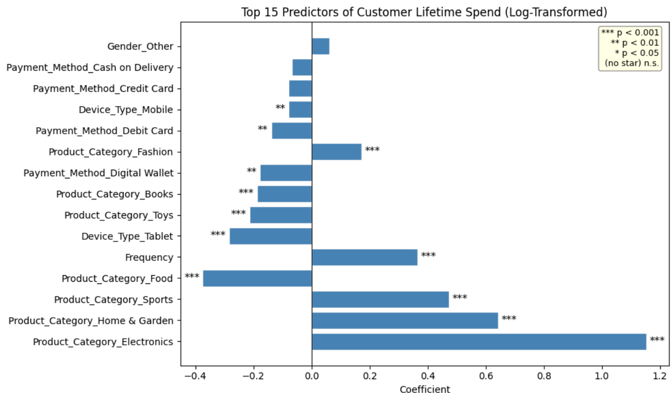
Figure 5: Top 15 predictors of log-transformed customer lifetime spend (OLS coefficients). Stars indicate statistical significance: *** p < 0.001 , ** p < 0.01 , * p < 0.05 .
