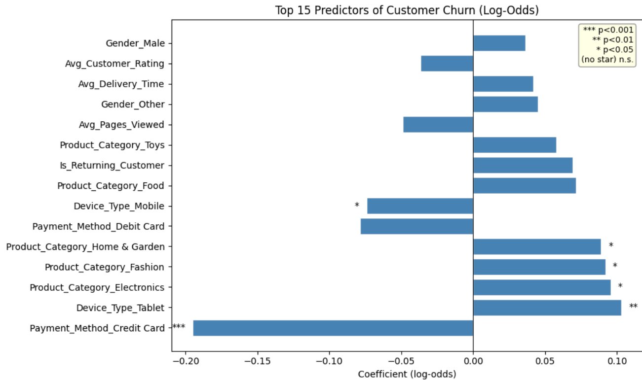
Figure 7: Top 15 predictors of customer churn (logistic regression log-odds, balanced model). Stars indicate statistical significance: *** p < 0.001 , ** p < 0.01 , * p < 0.05 .
