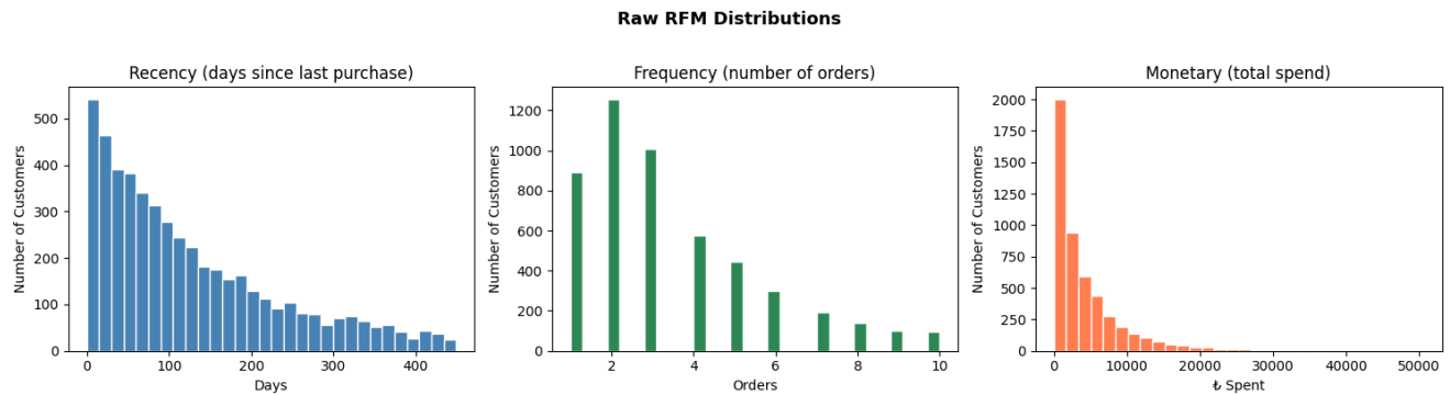
Figure 1: Raw RFM distributions (Recency, Frequency, Monetary) across 5,000 customers.
