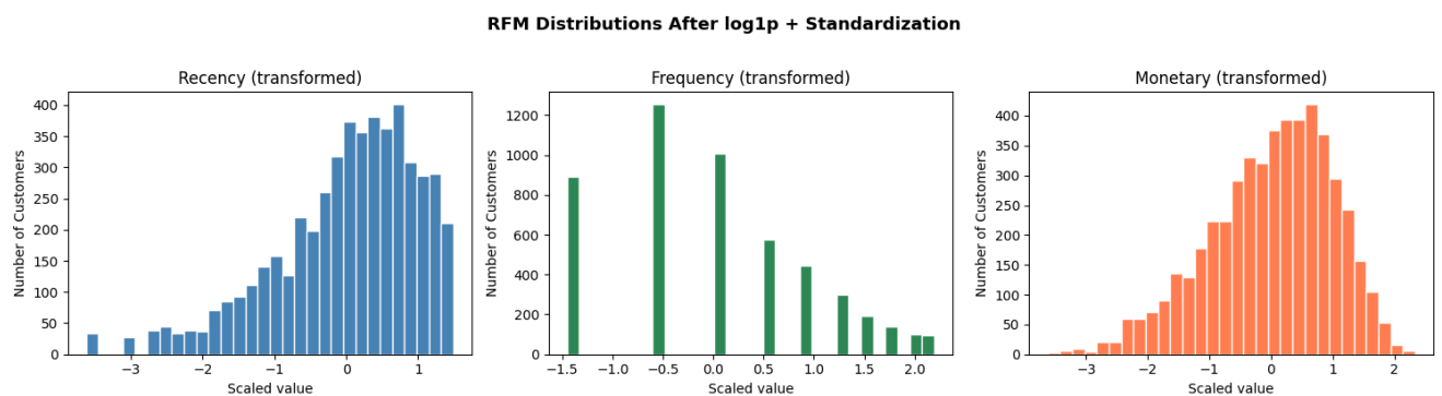
Figure 2: RFM distributions after log1p transformation and standardization.
