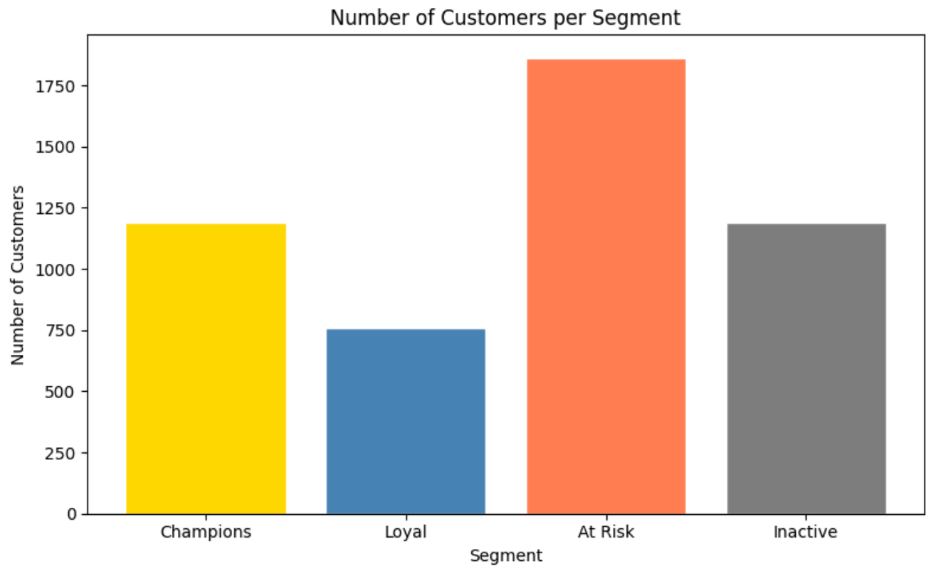
Figure 4: Bar chart showing the number of customers in each segment.
