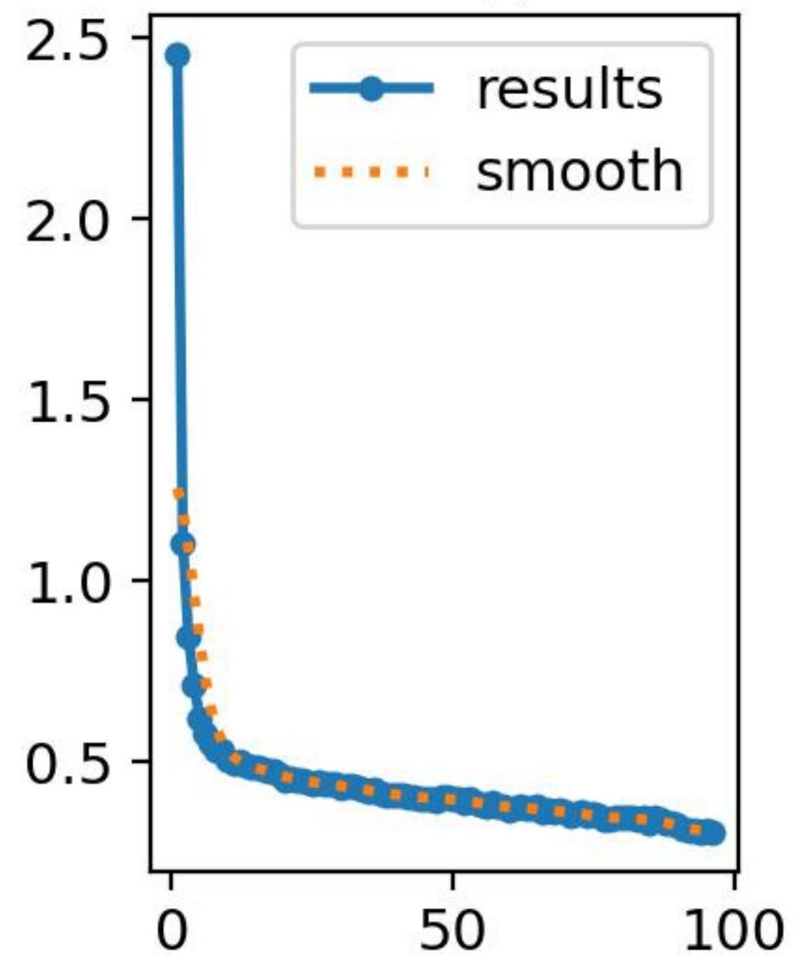
train/cls_loss
