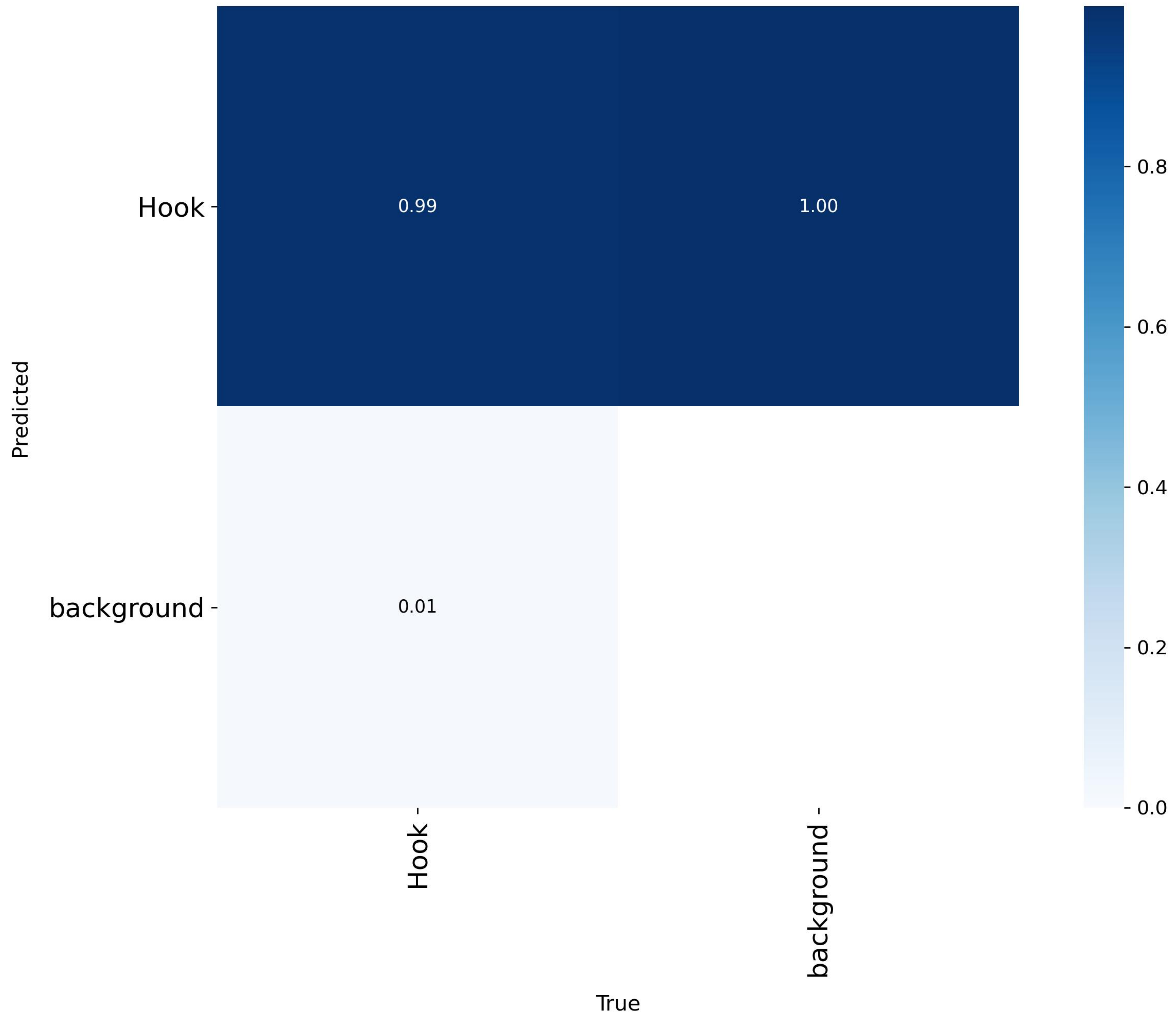
Confusion Matrix Normalized
