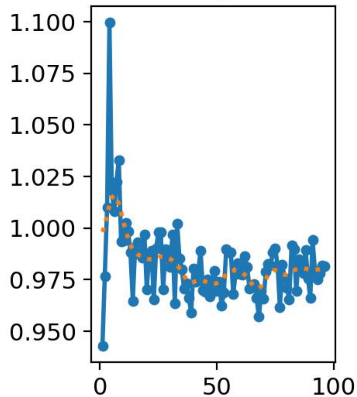
val/dfl_loss
