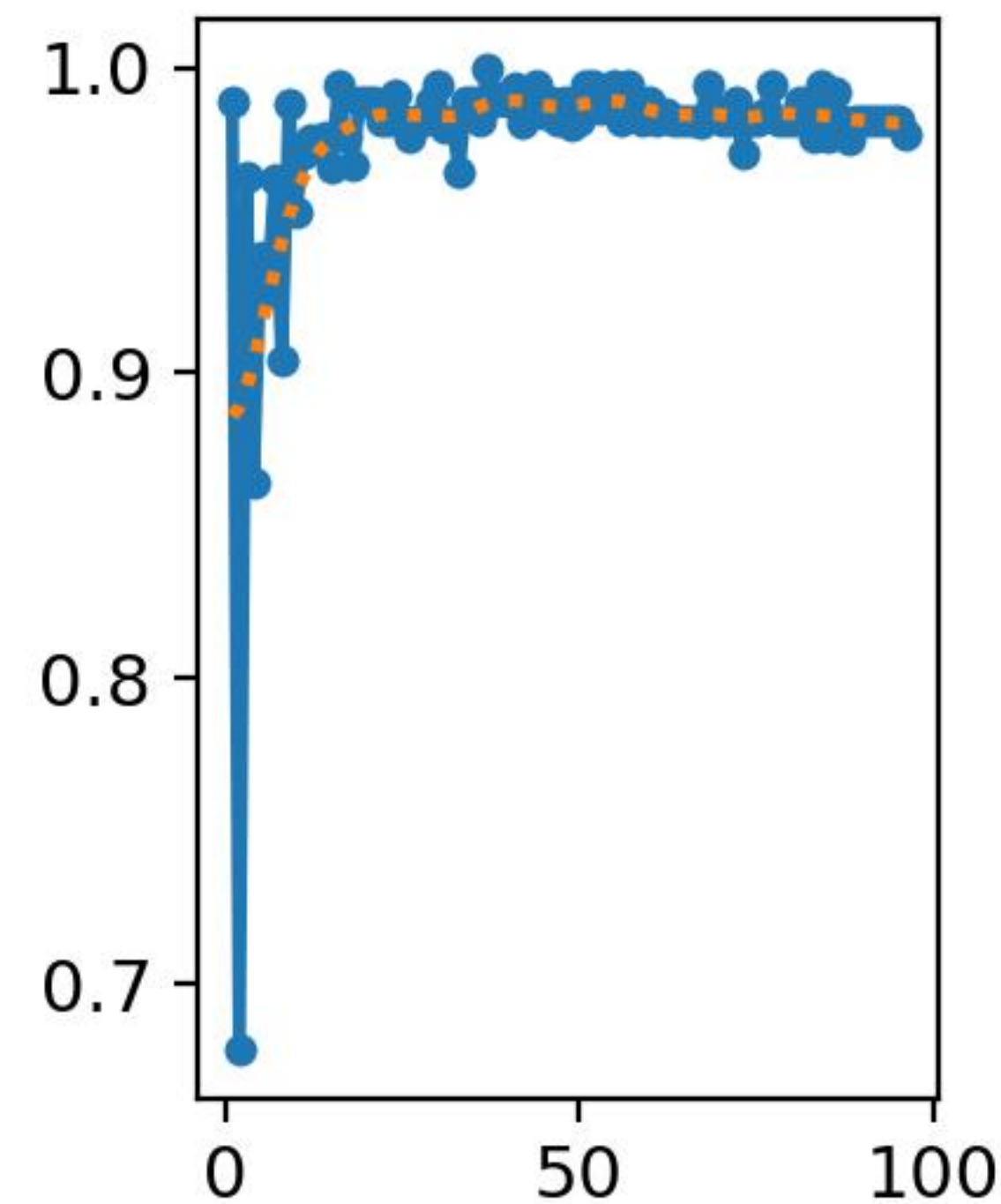
metrics/recall(B)
