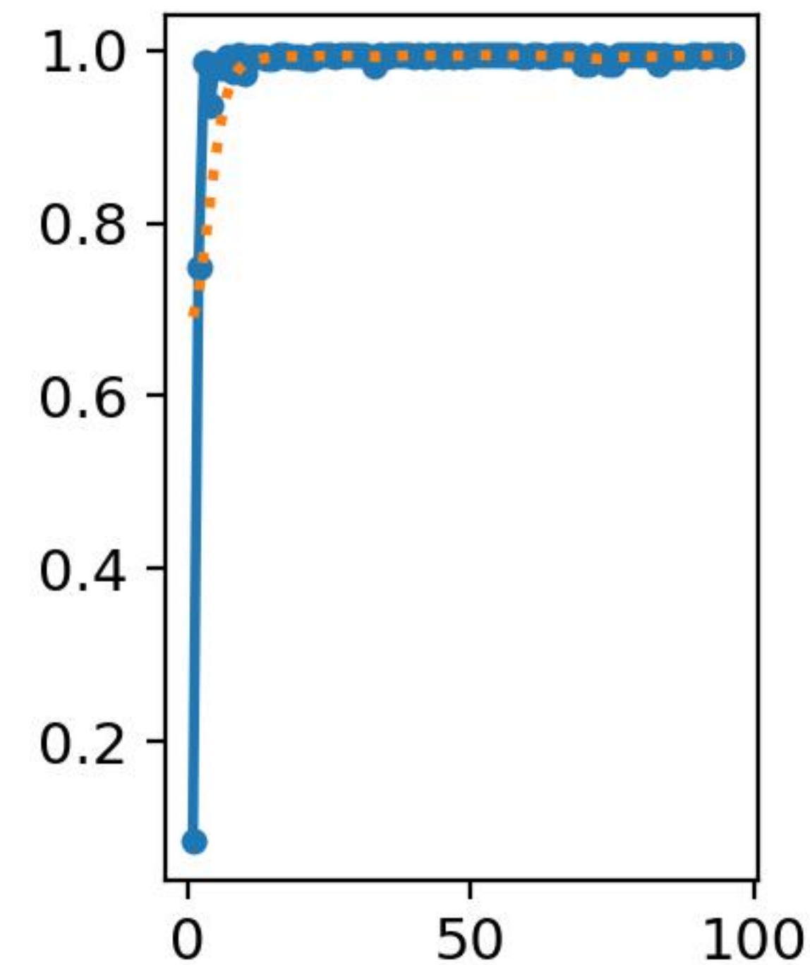
metrics/mAP50(B)
