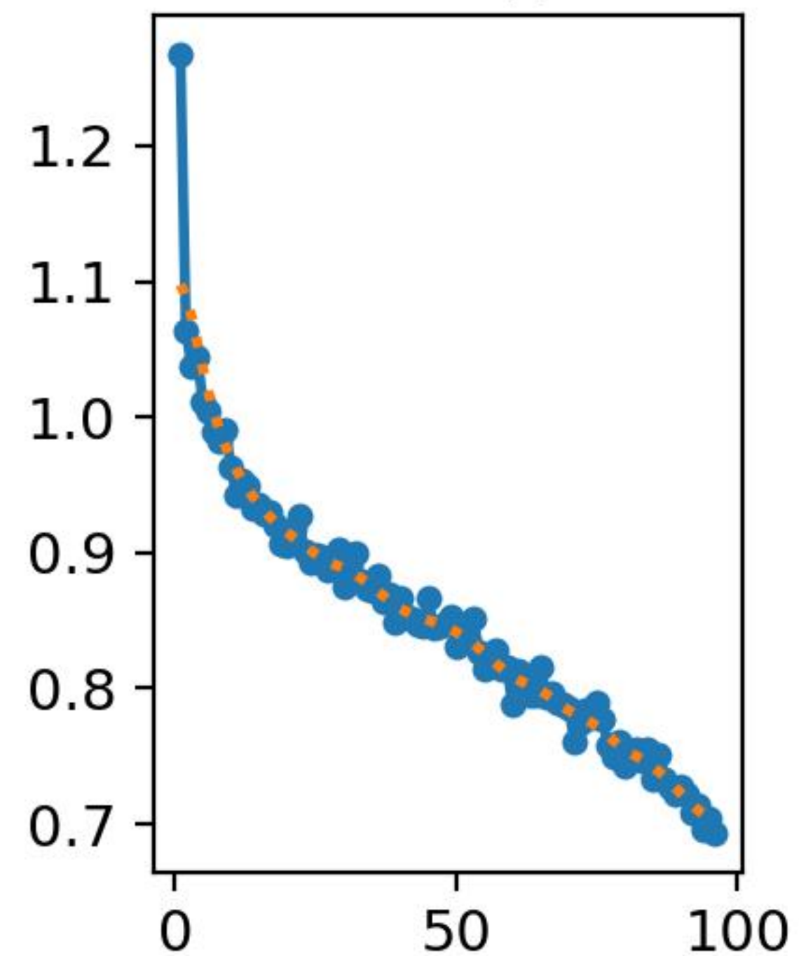
train/box_loss
