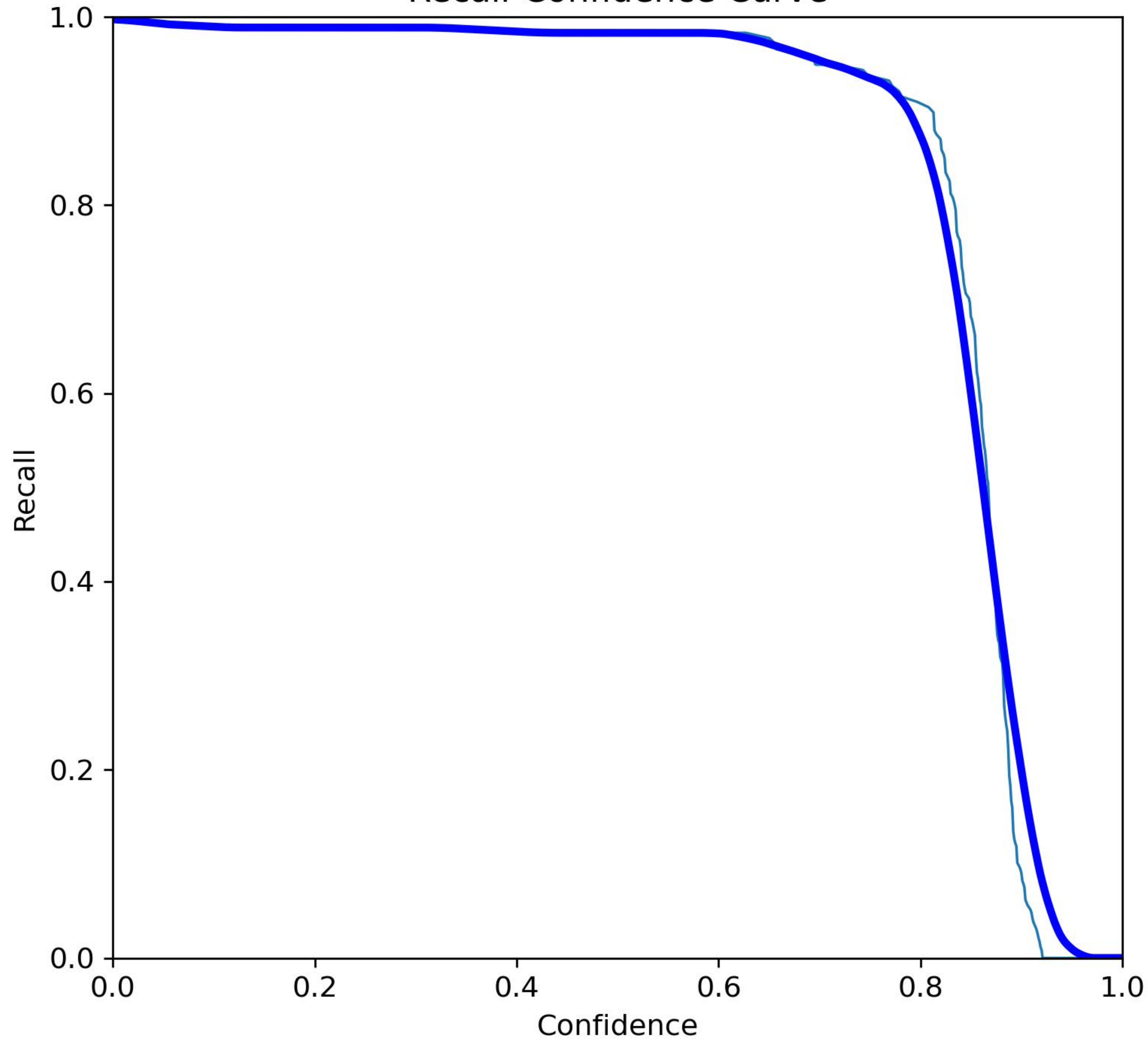
Recall-Confidence Curve
