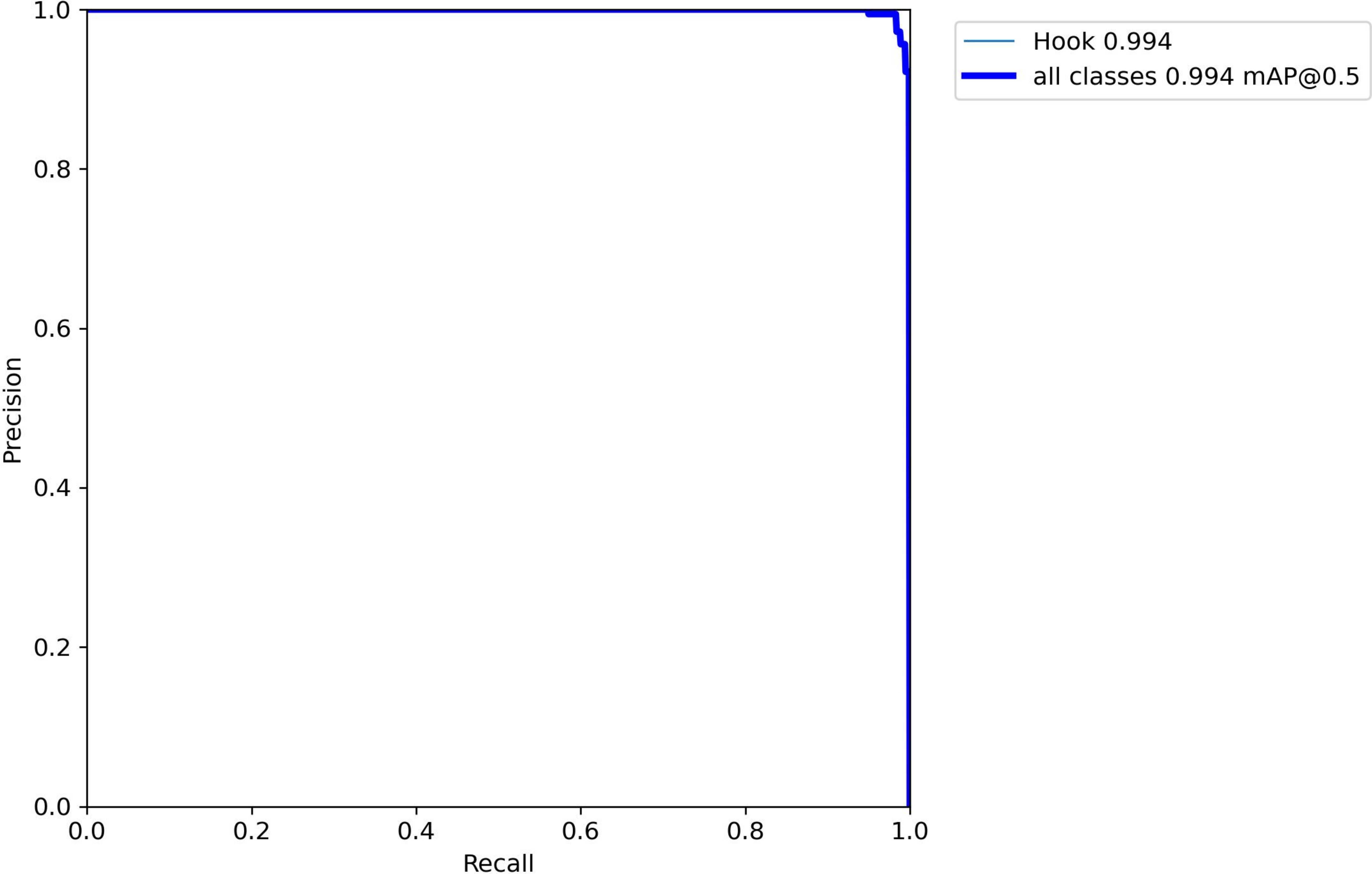
Precision-Recall Curve
