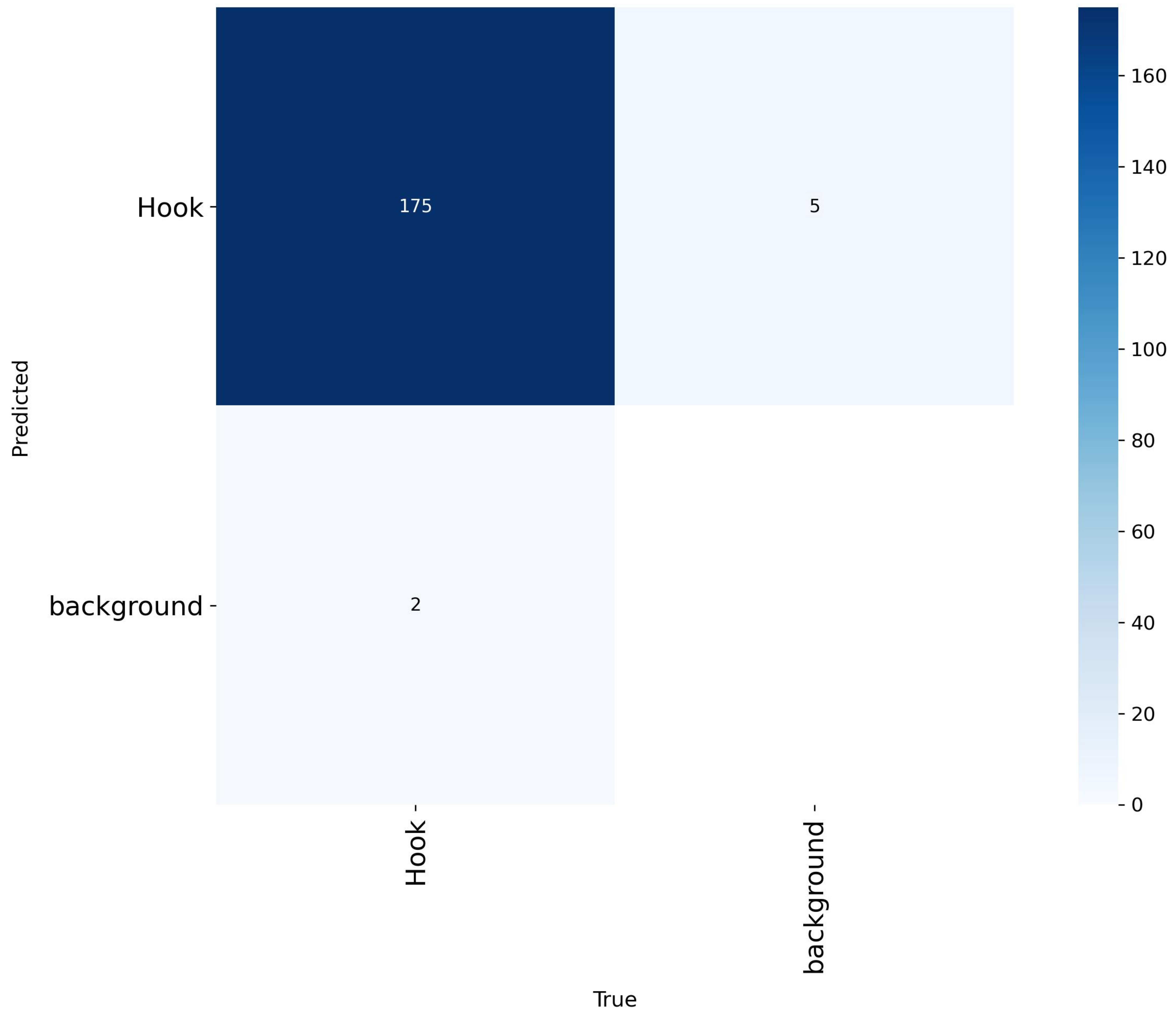
Confusion Matrix
