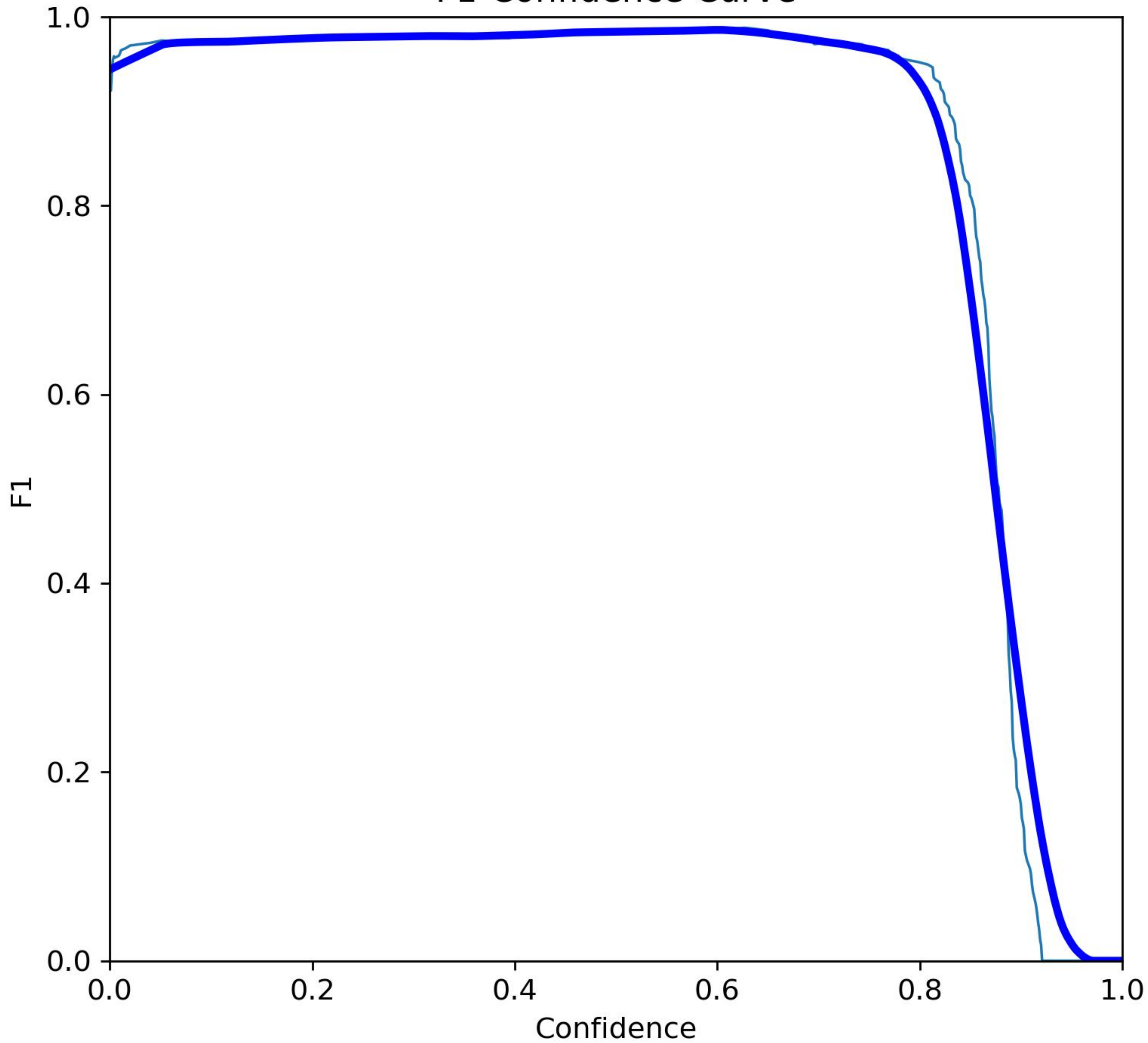
F1-Confidence Curve
