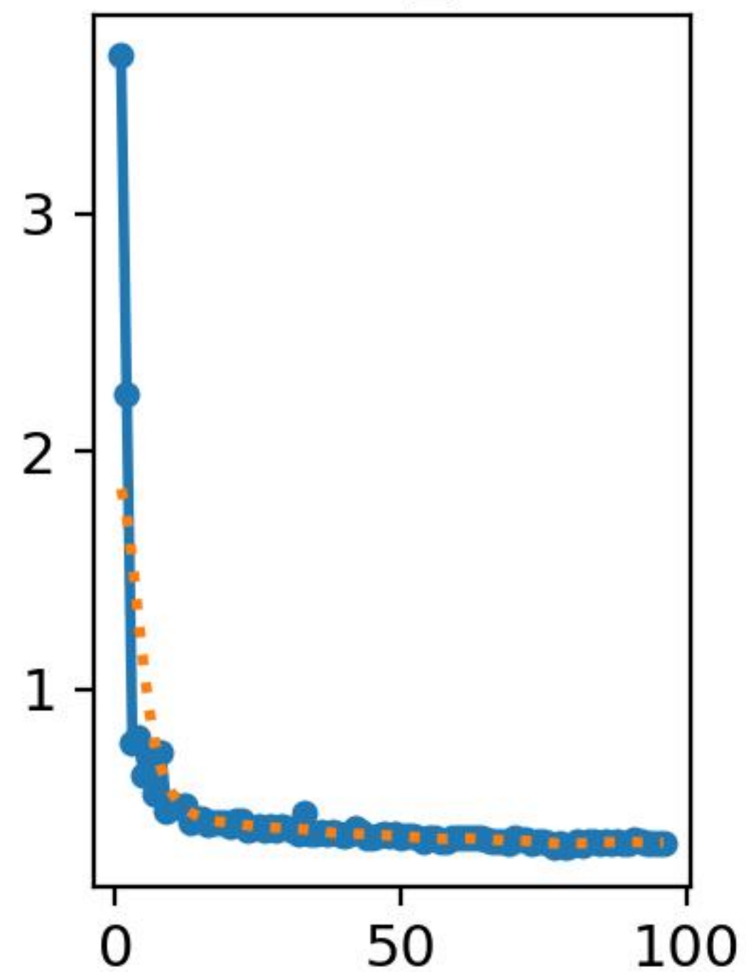
val/cls_loss
