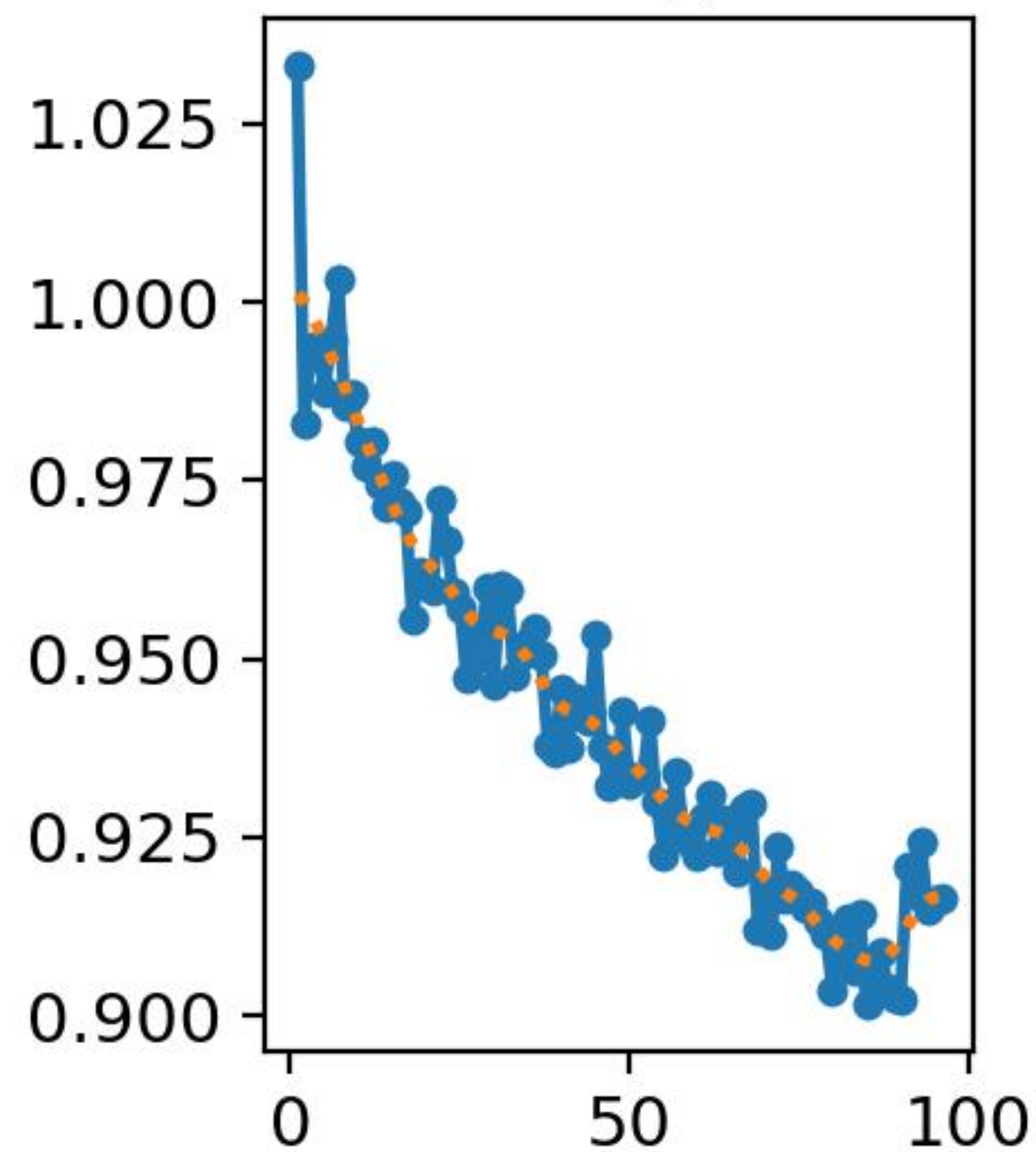
train/dfl_loss
