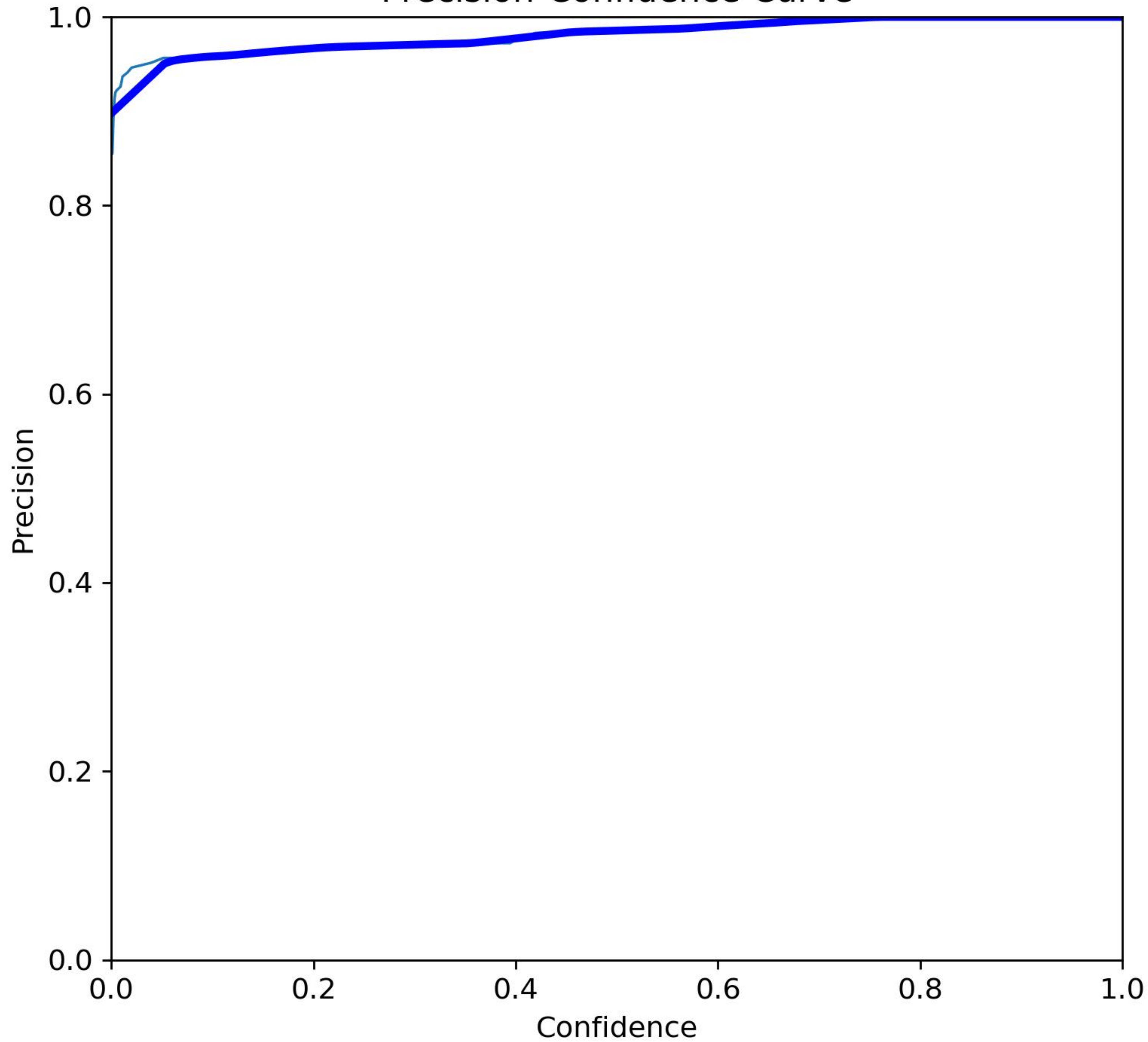
Precision-Confidence Curve
