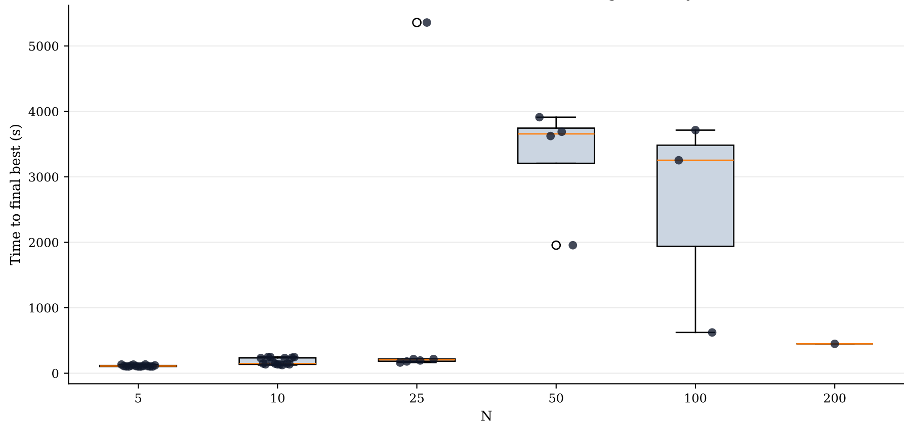
Distribution of time to final best feasible configuration by N
