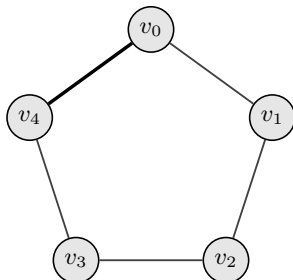
bold edge v_4v_0 is the forced clash
