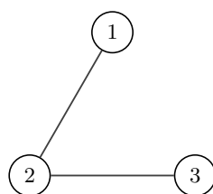
subgraph, not induced
