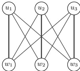
K_{3,3} : bold perfect matching forces C = all 6 vertices, yet top row alone covers
