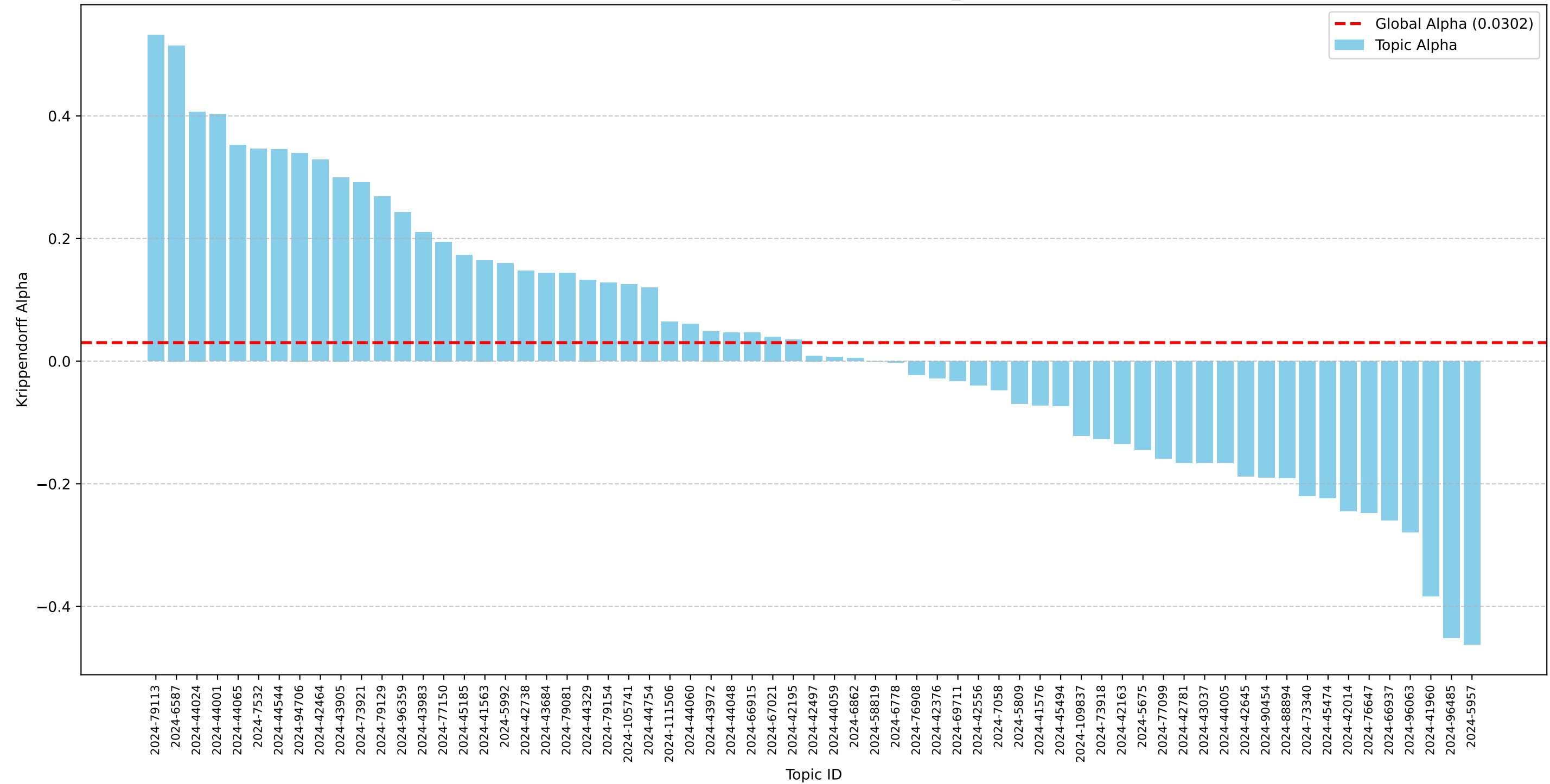
Krippendorff Alpha by Topic: coherence_logical
