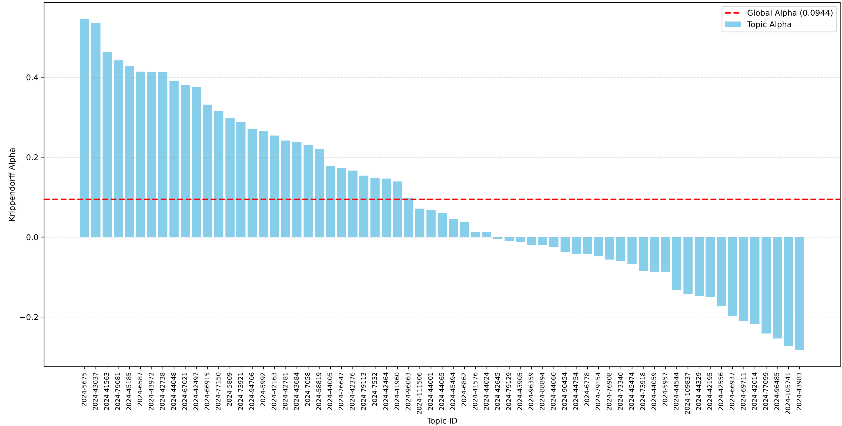
Krippendorff Alpha by Topic: coherence_stylistic
