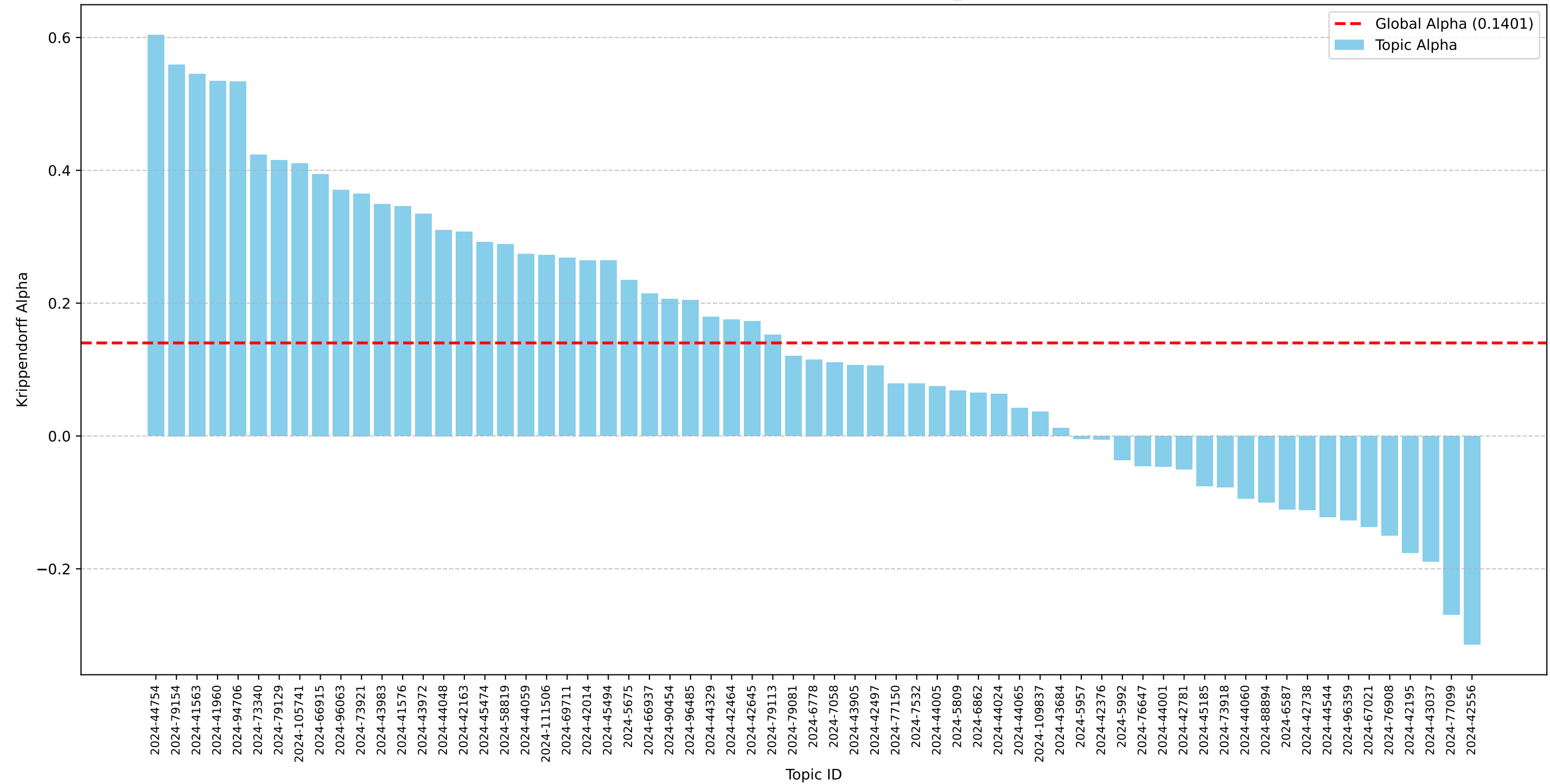
Krippendorff Alpha by Topic: coverage_deep
