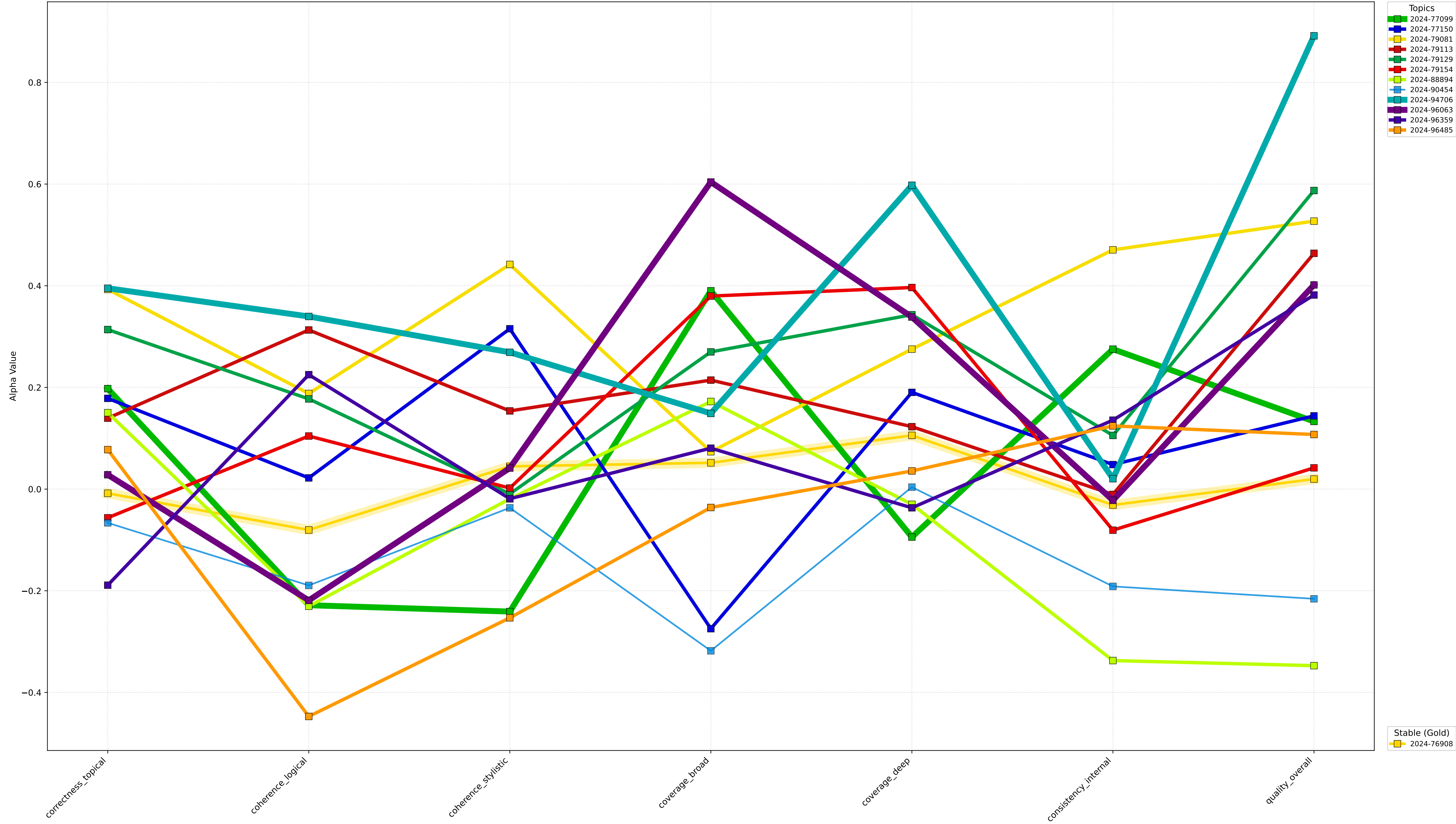
Krippendorff Alpha (Topics 53-65)
