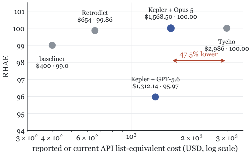
Figure 5: Score against disclosed or current API list-equivalent cost. Kepler’s $1,568.50 is the lowest disclosed bill among the 100.00 systems reviewed; Tycho reports $2,986, while AVO and VISTA do not publish comparable costs. Retrodict and baseline1 occupy cheaper, lower-scoring points. Pricing and accounting methods differ, so this is a disclosed frontier rather than a controlled efficiency experiment.
