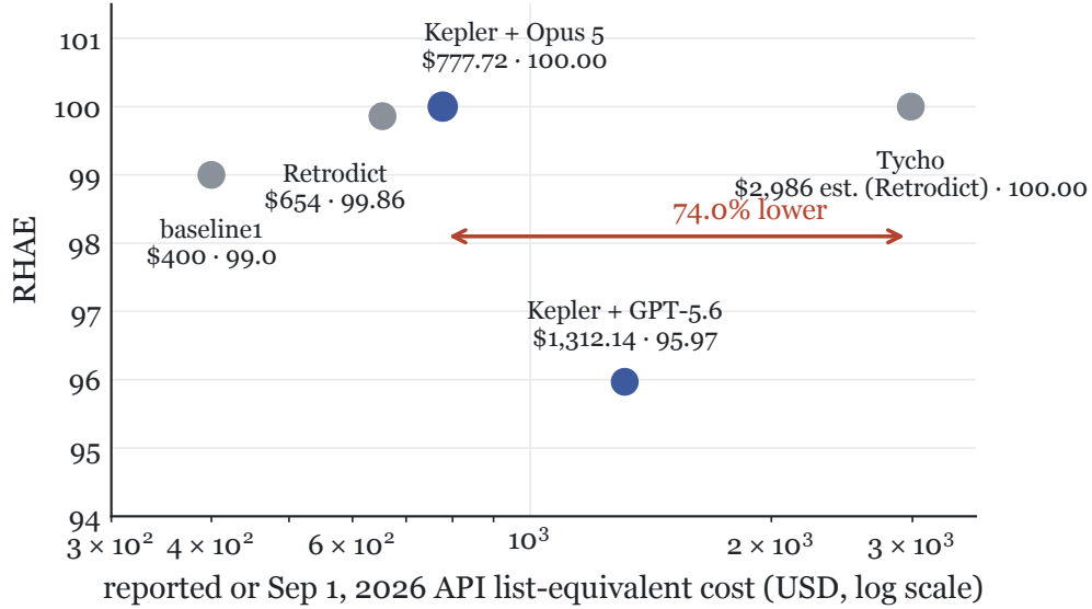
Figure 5: Score against disclosed or September 1, 2026 API list-equivalent cost. Kepler’s $777.72 is 74.0% below the $2,986 API-equivalent estimate Retrodict published for Tycho; Tycho discloses no cost of its own, and AVO and VISTA publish none. Retrodict and baseline1 occupy cheaper, lower-scoring points. Pricing and accounting methods differ, and most of the field reports nothing, so this is a sparse disclosure frontier rather than a controlled efficiency experiment.
