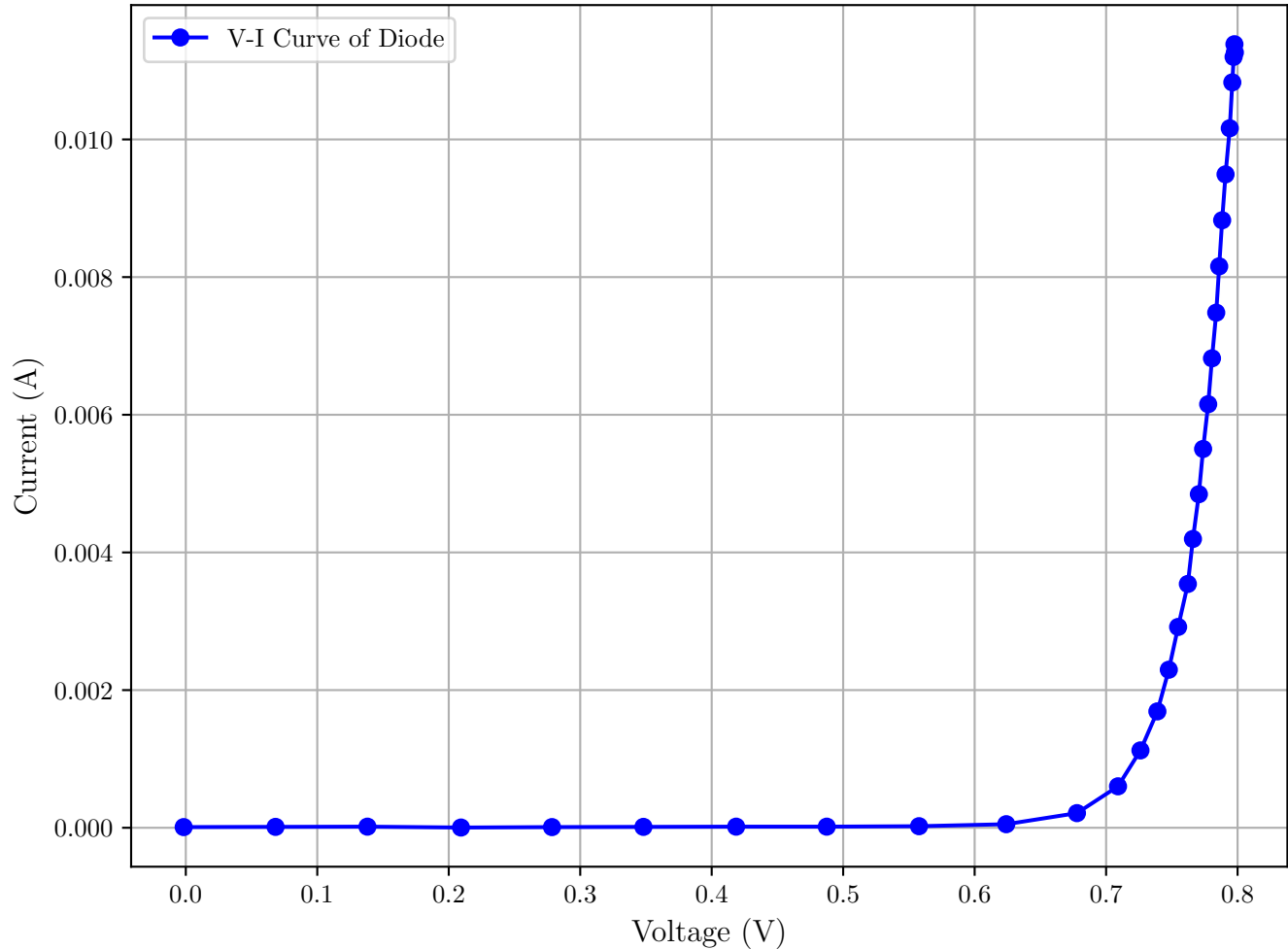
Voltage-Current Characteristics of Zener Diode
