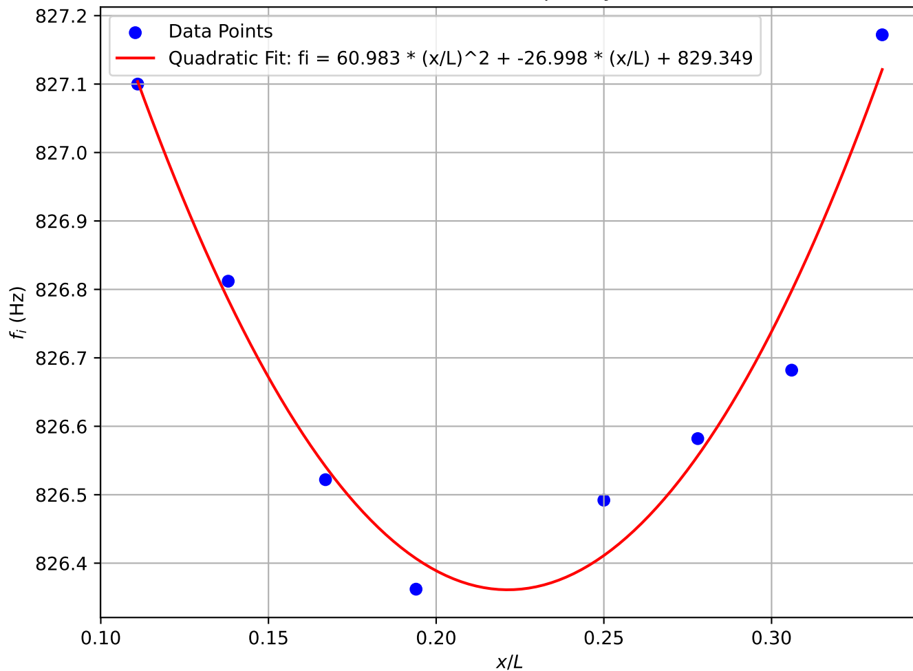
Quadratic Fit of Resonant Frequency vs Position Ratio
