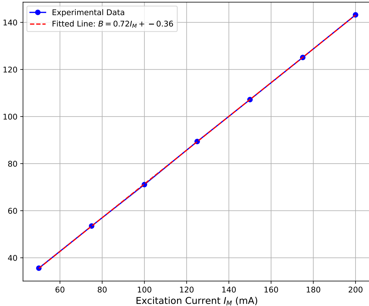
Magnetic Flux Density B vs Excitation Current I_M
