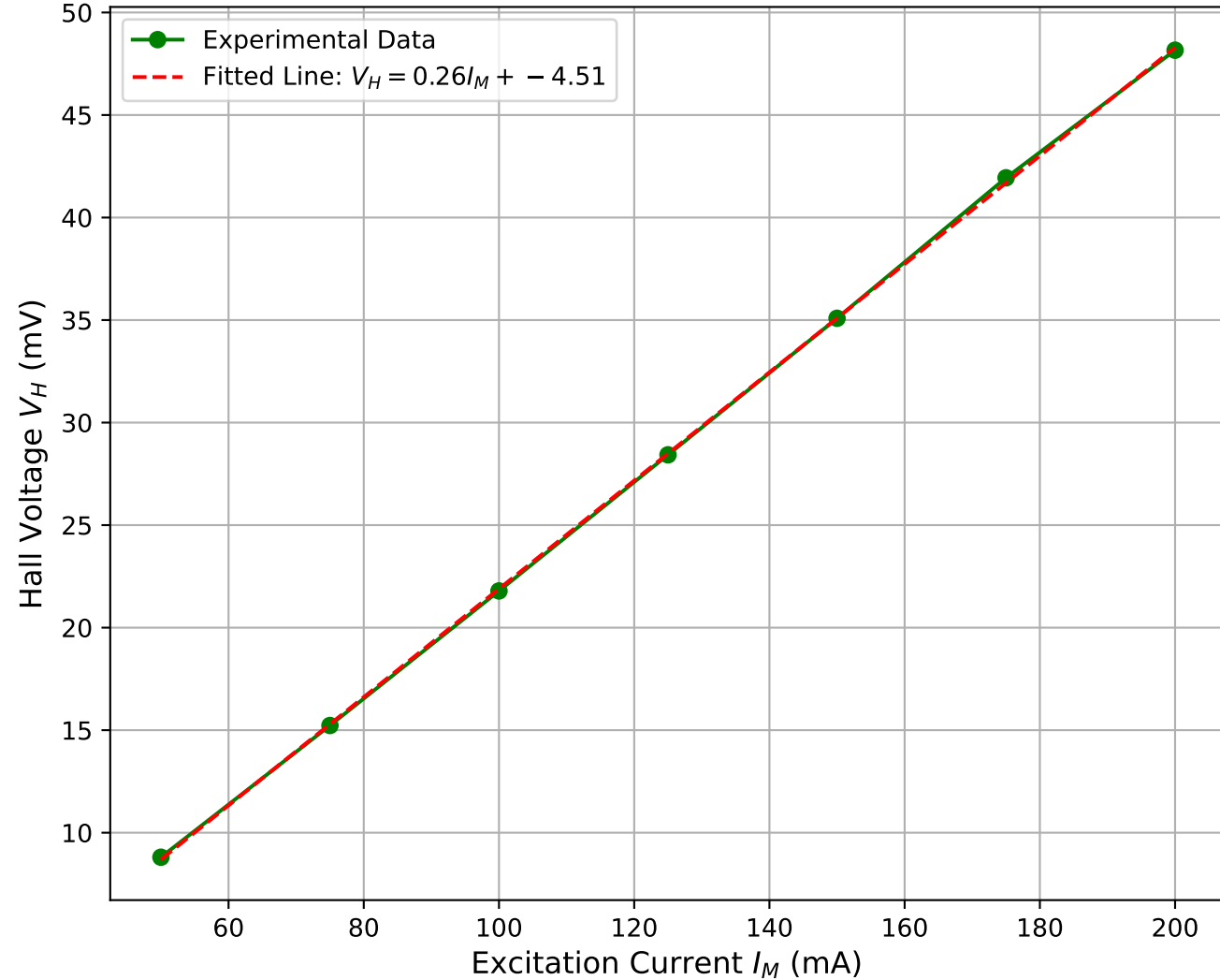
Hall Voltage V_H vs Excitation Current I_M (AC)
