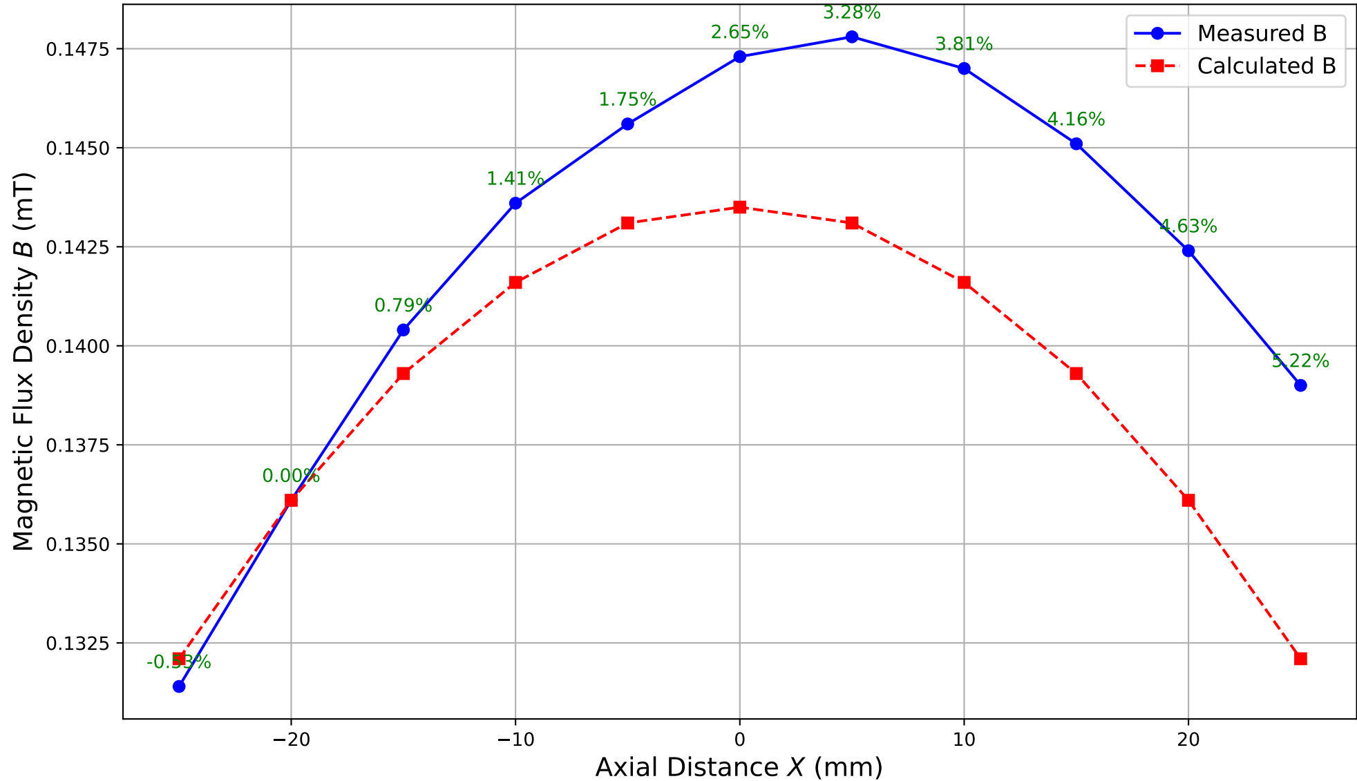
Magnetic Flux Density B vs Axial Distance X
