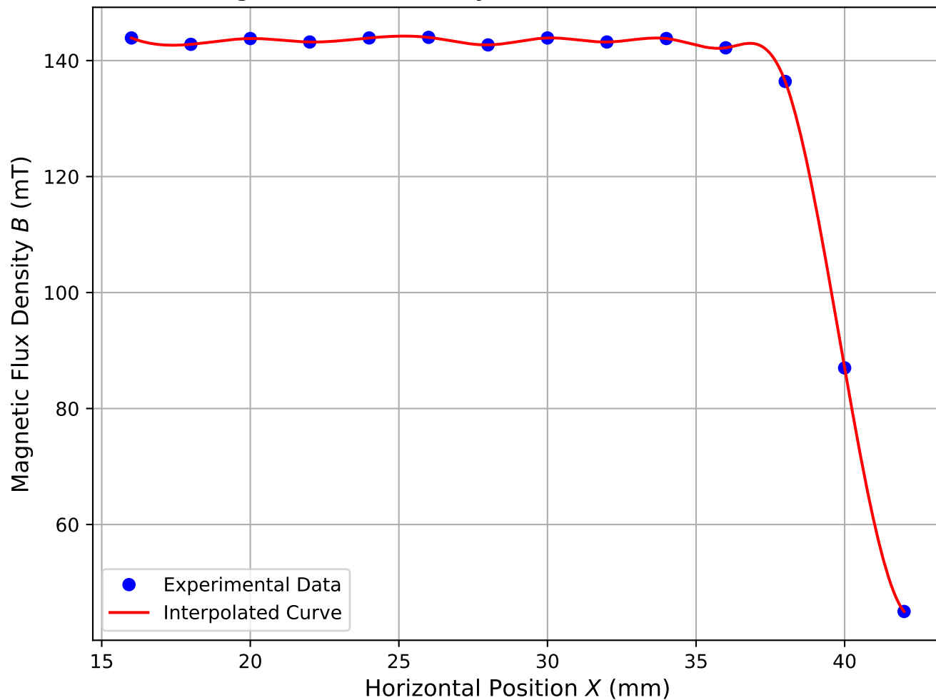
Magnetic Flux Density B vs Horizontal Position X
