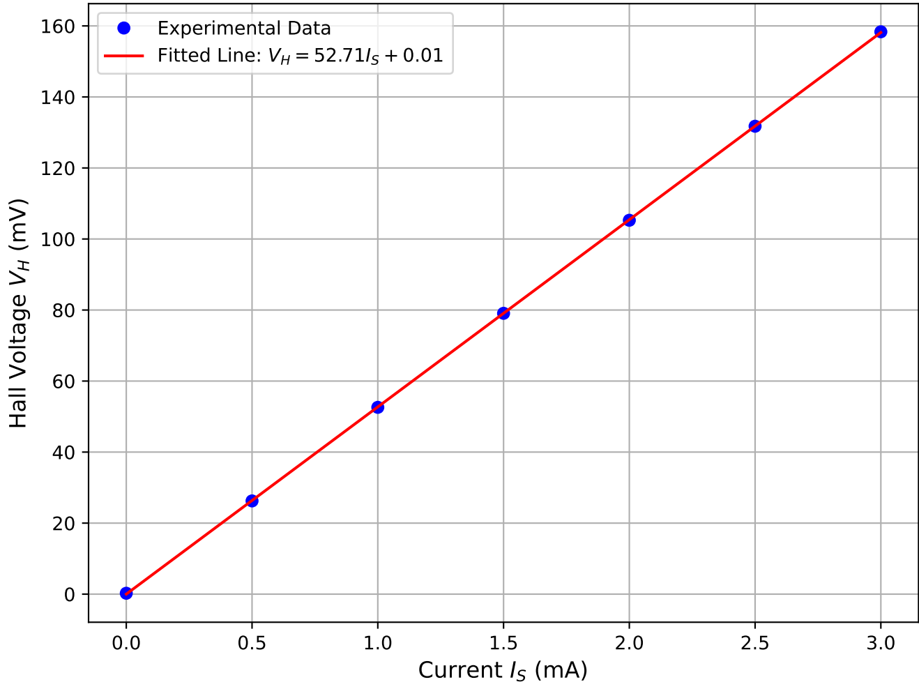
Hall Voltage V_H vs Current I_S
