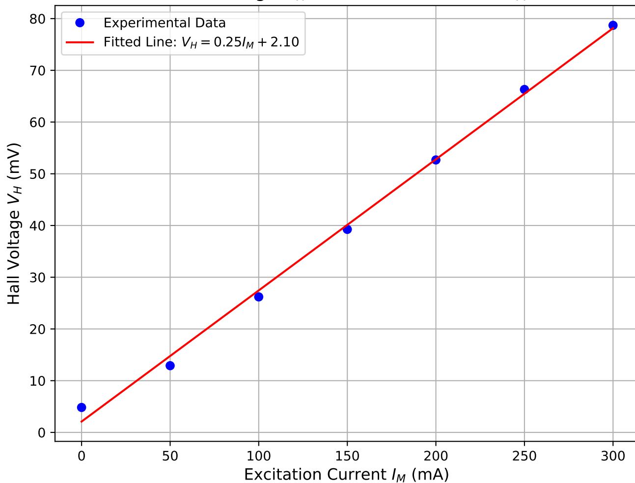
Hall Voltage V_H vs Excitation Current I_M
