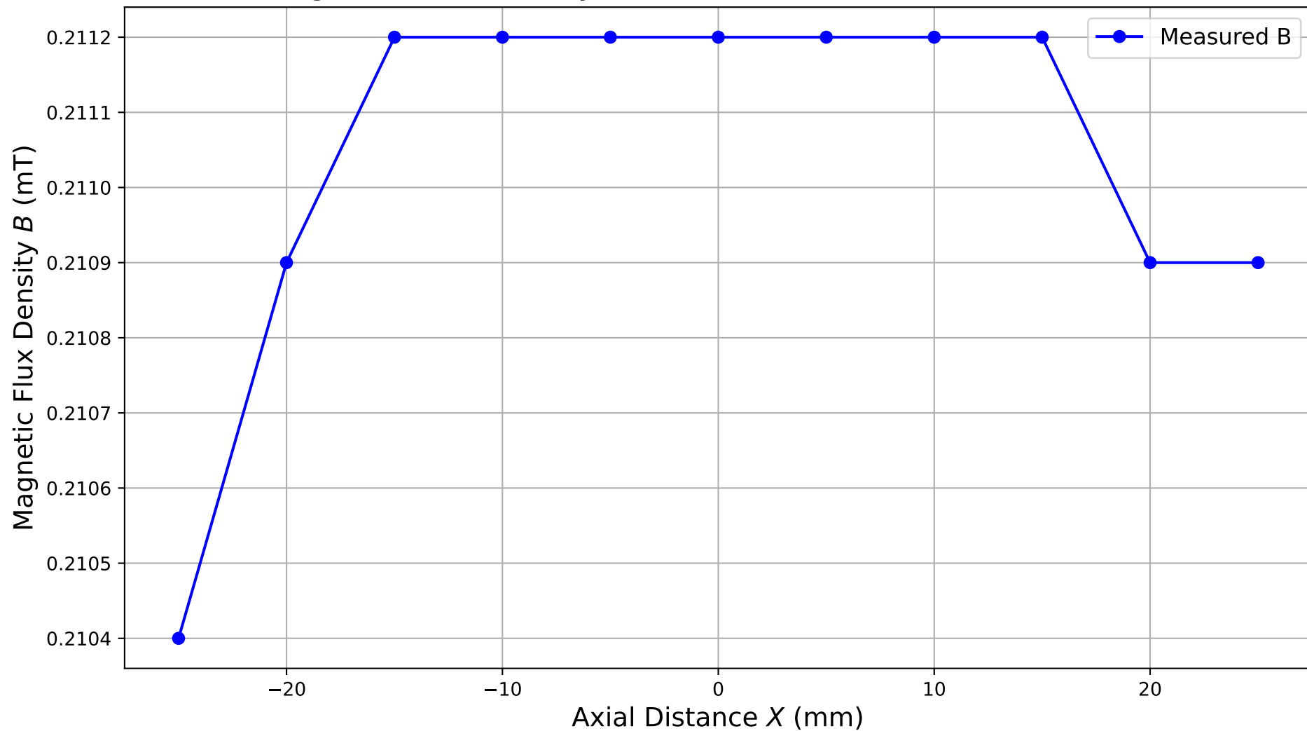
Magnetic Flux Density B vs Axial Distance X (Helmholtz Coil)
