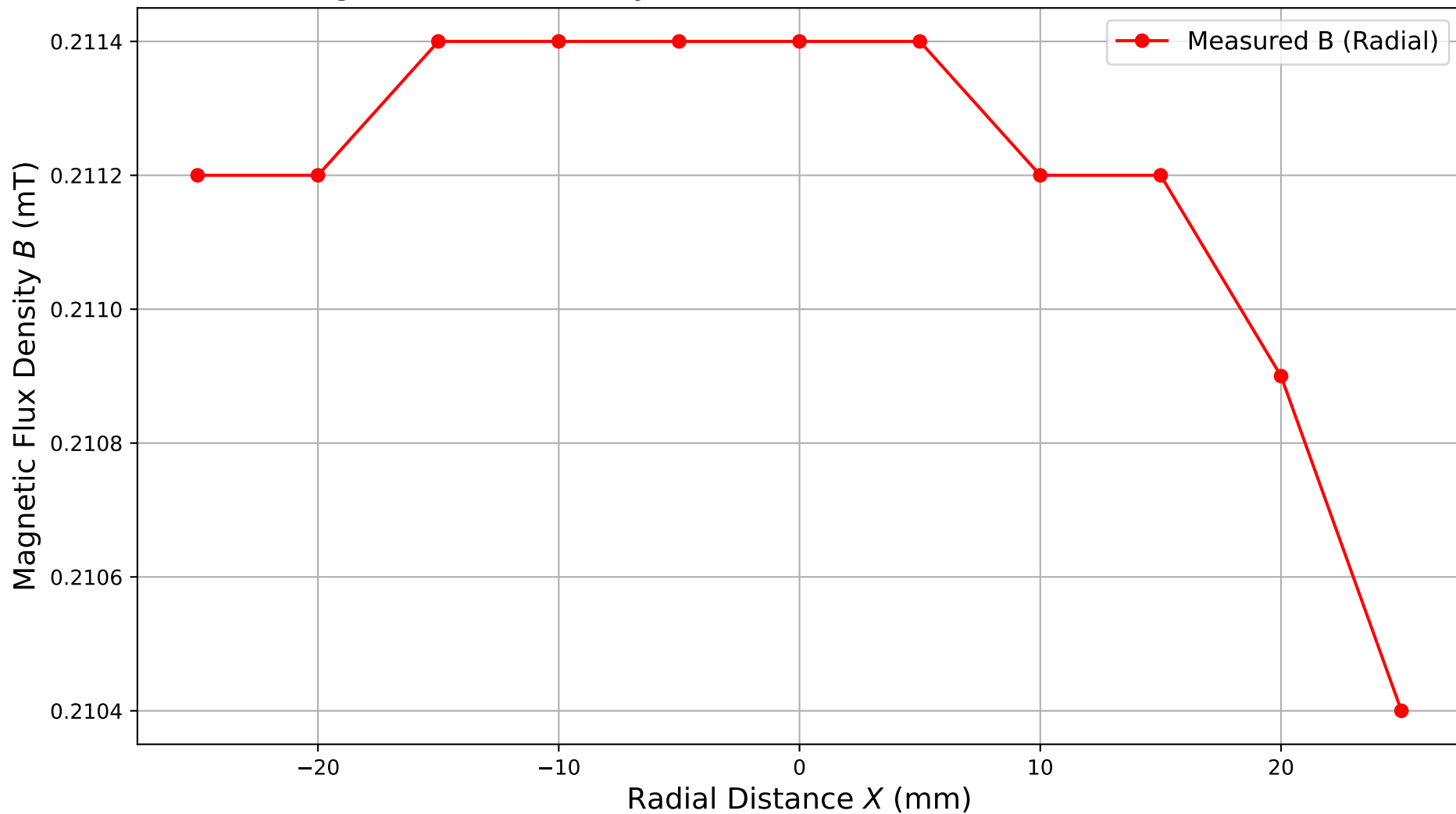
Magnetic Flux Density B vs Radial Distance X (Helmholtz Coil)
