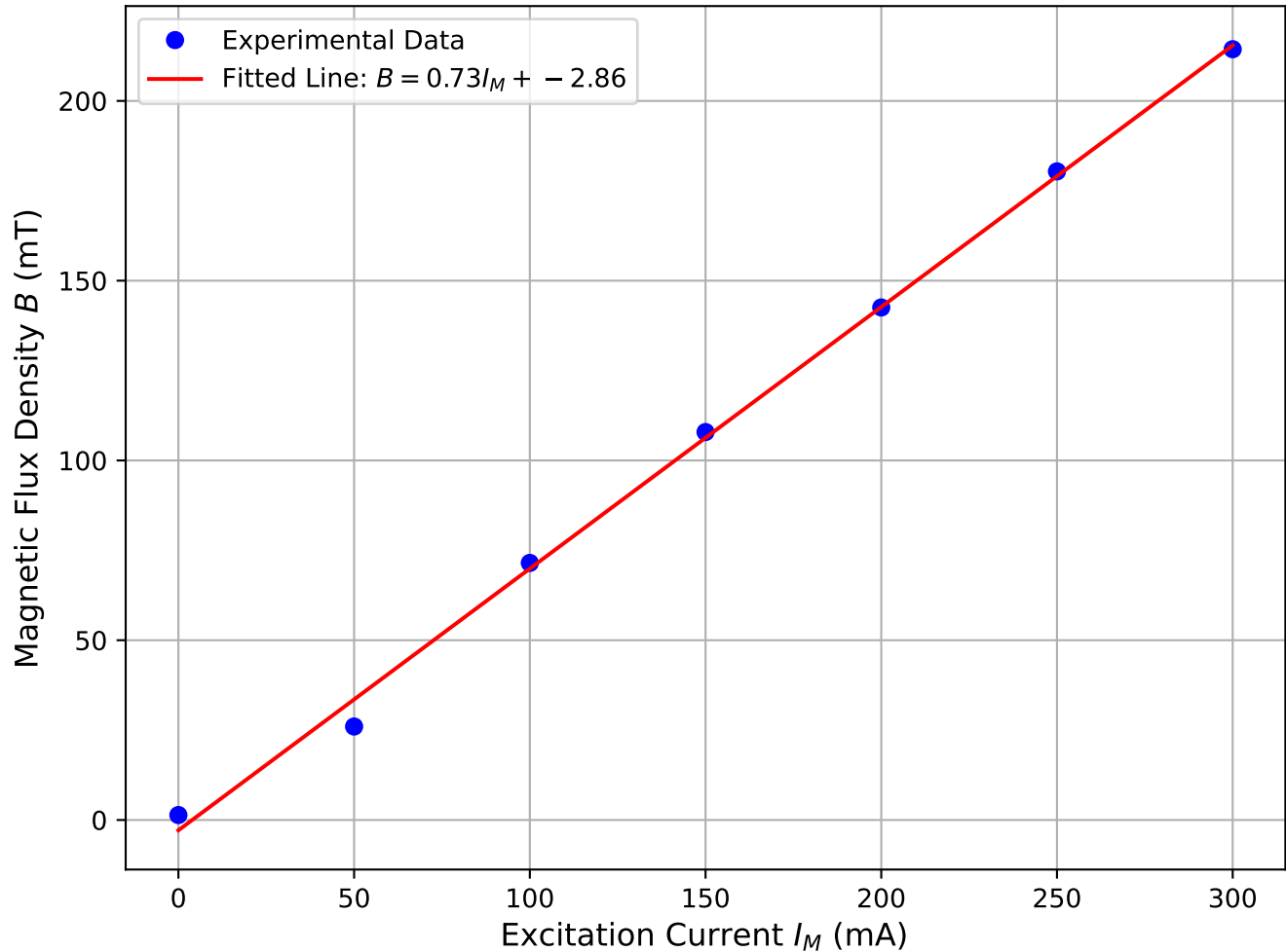
Magnetic Flux Density B vs Excitation Current I_M
