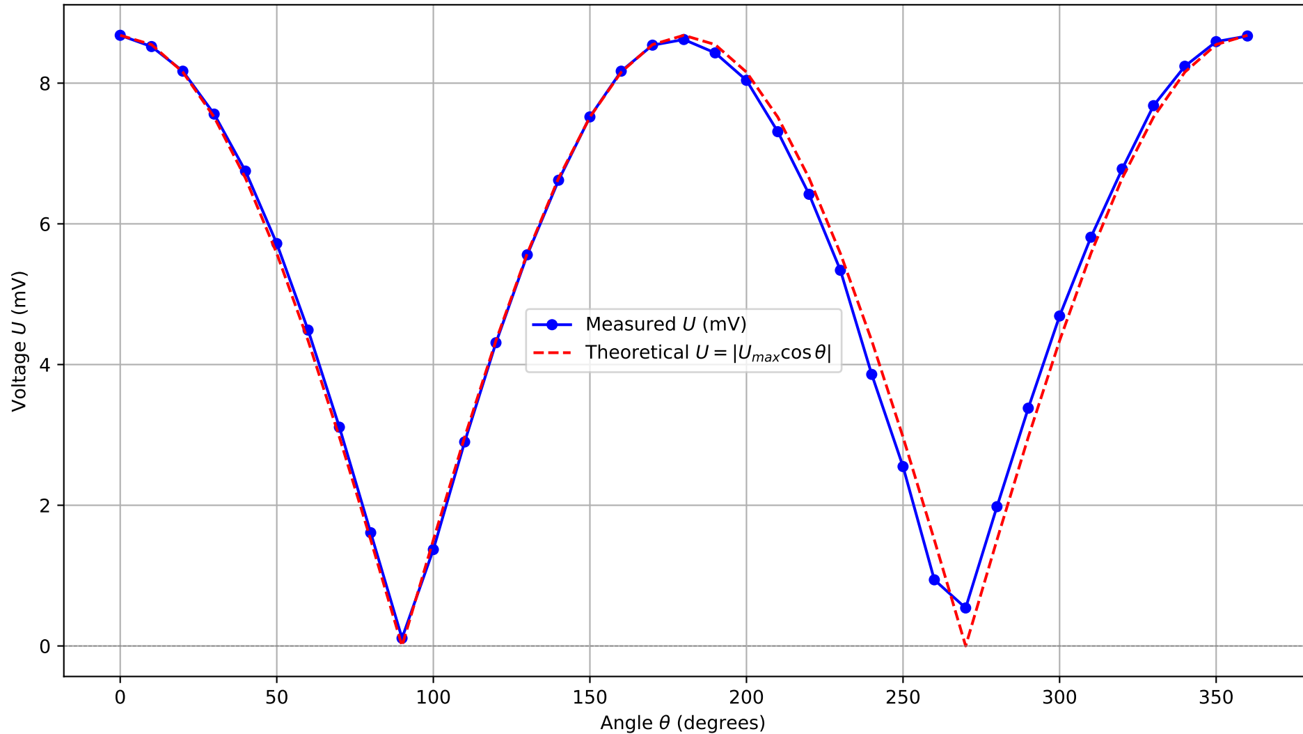
Induced Voltage vs Coil Angle
