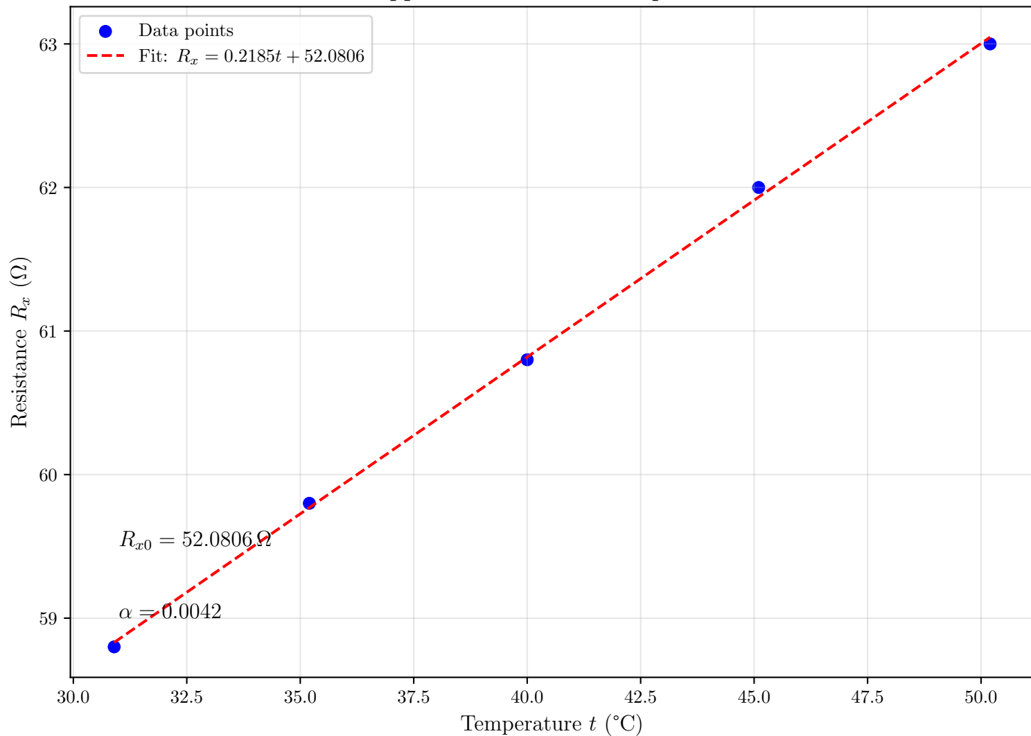
Copper Resistance vs Temperature
