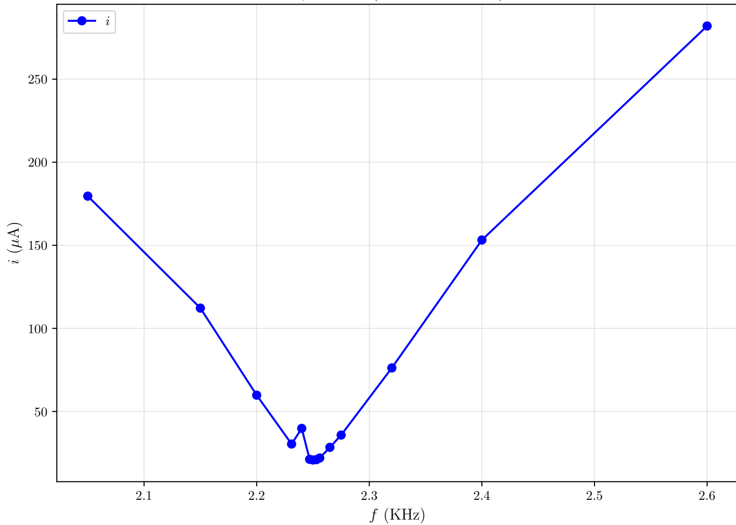
i - f Curve (Parallel Circuit)
