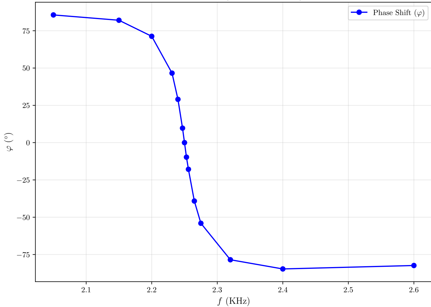
\varphi - f Curve (Parallel Circuit)
