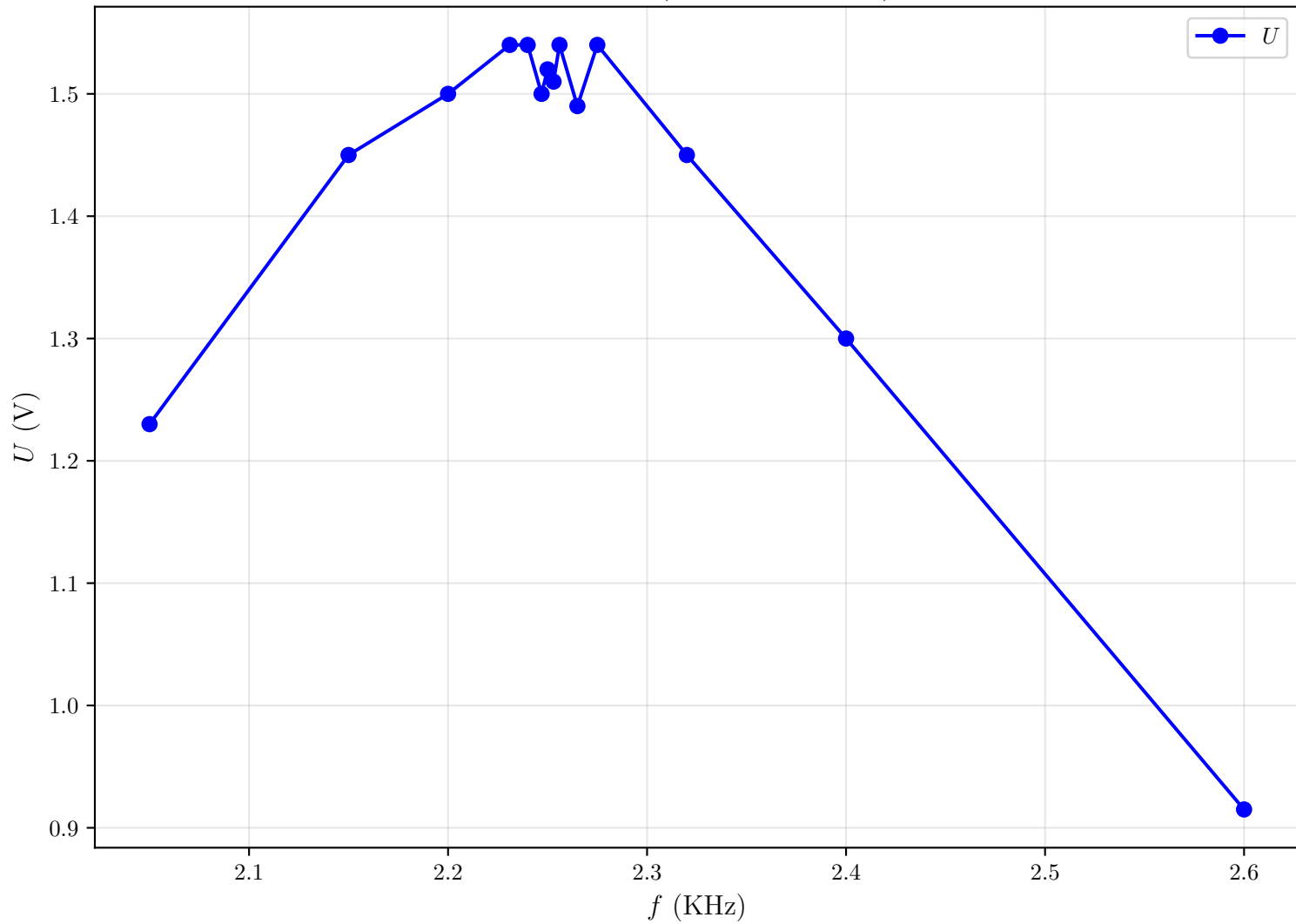
U - f Curve (Parallel Circuit)
