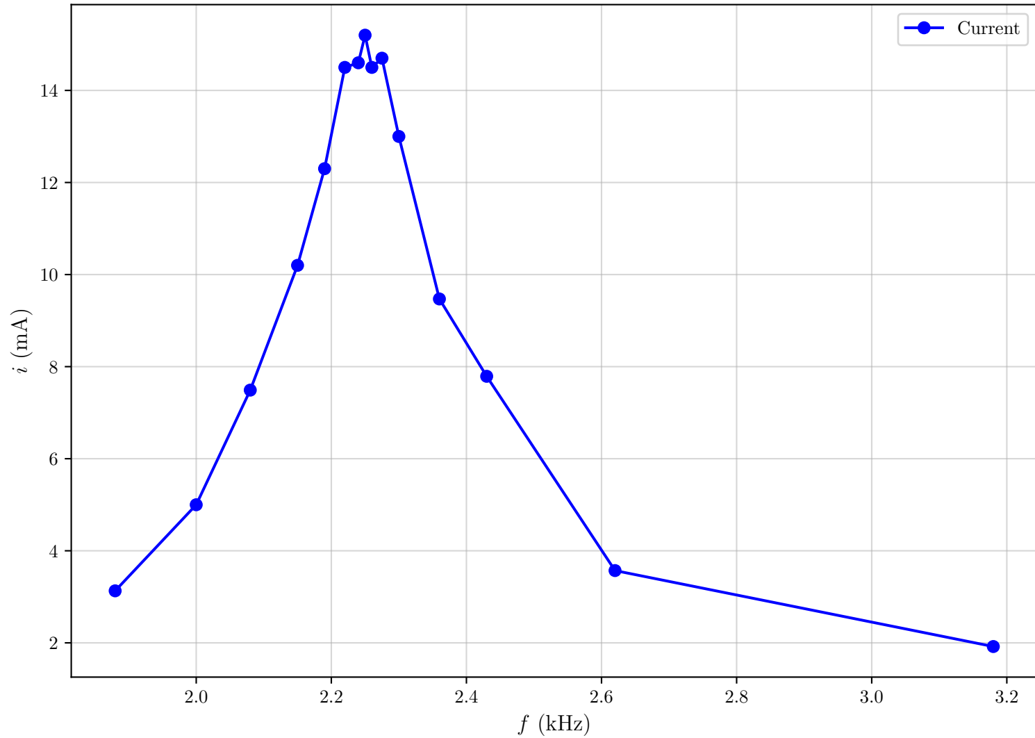
i - f Curve for Series Circuit
