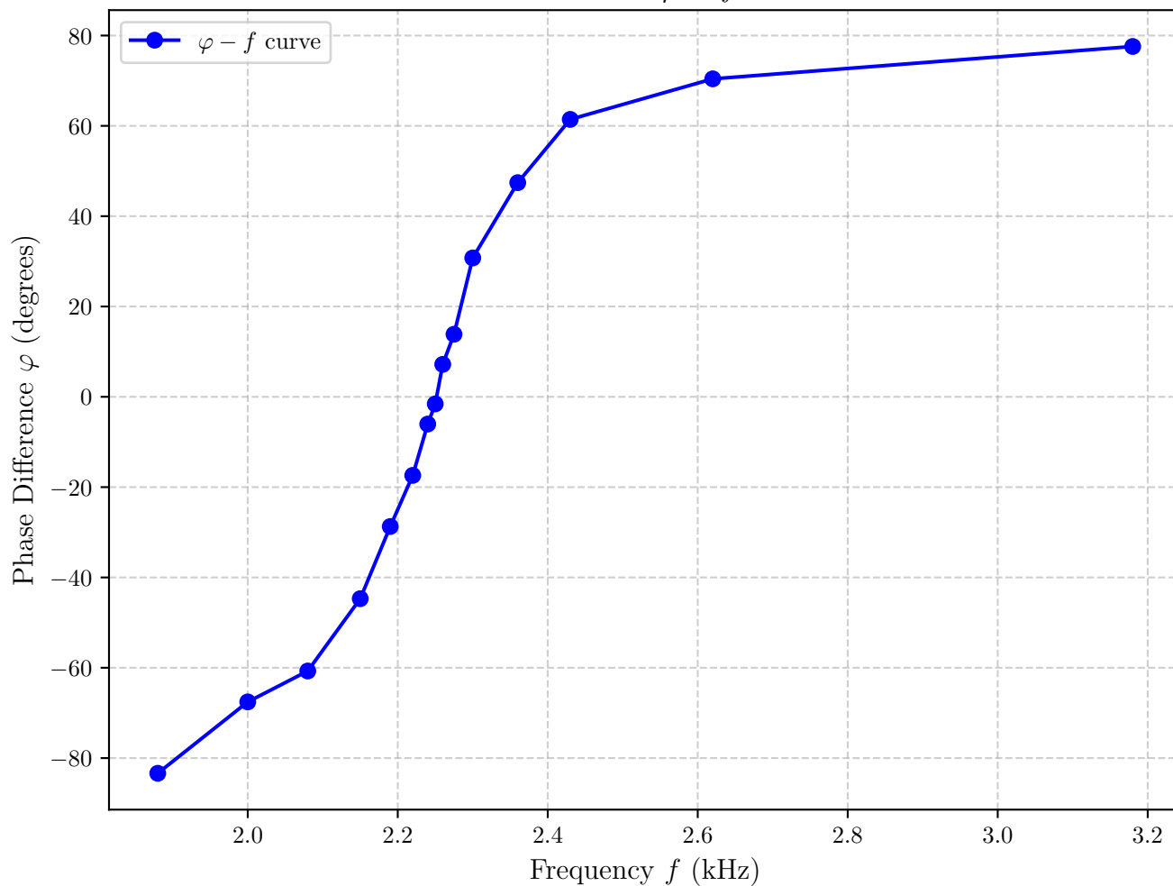
Series Circuit \varphi - f Curve
