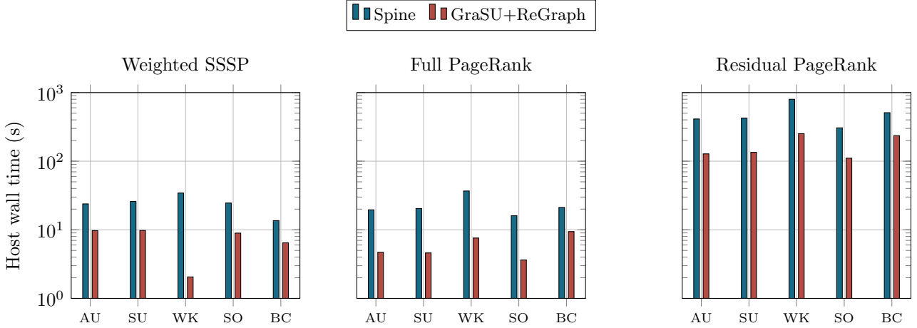
Figure 9: Observed simulator host runtime for the archived insertion-batch-8 runs. Every dataset has 8,192 base edges, while vertex counts vary from 2,004 to 10,326 as listed in Table 1. Each bar is one previously executed child-process observation from a parallel experiment matrix, not a repeated controlled benchmark. These values are engineering evidence for simulator-throughput planning and are not accelerator latency.
