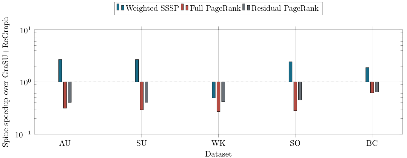
Figure 2: Insert-batch-8 E2E comparison on five compact temporal slices. Values above one favor Spine; values below one favor GraSU+ReGraph.
