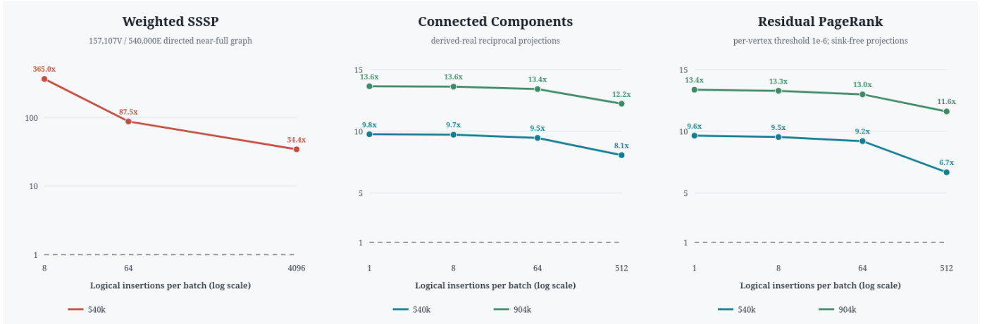
Figure 1: Correctness-gated Spine speedup over K=1 GraSU+ReGraph. Weighted SSSP uses the directed 157,107-vertex, 540,000-edge near-full AskUbuntu graph. CC and per-vertex-threshold residual PageRank use deterministic reciprocal projections at 540,000 and 903,774 edge records. CC and residual updates are nested component bridges rather than original temporal events. All rows pass independent algorithm oracles and cross-system work checks.
