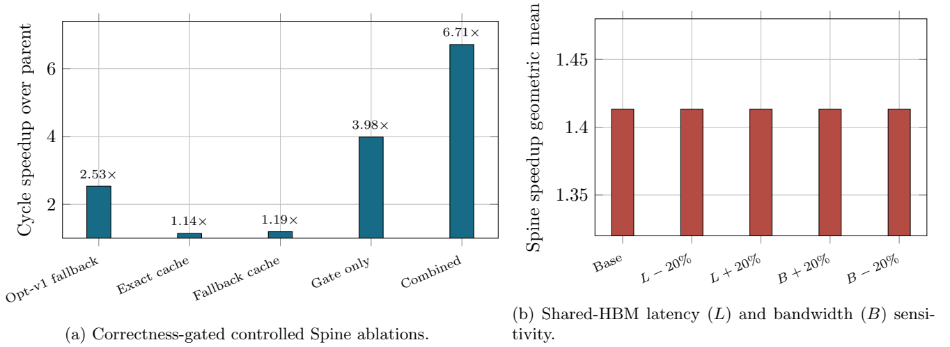
Figure 13: Optimization scope and robustness. Opt-v1 reuses the launch-level cache only in active-capacity fallback. Opt-v2 adds a finite source-page working set and expands the exact-path active-record gate; the 50K “gate only” and “combined” bars are mechanism ablations, not the paper-scale three-algorithm mean. The HBM panel covers 12 correctness-gated pairs per profile and has zero strict architecture-ranking inversions.
