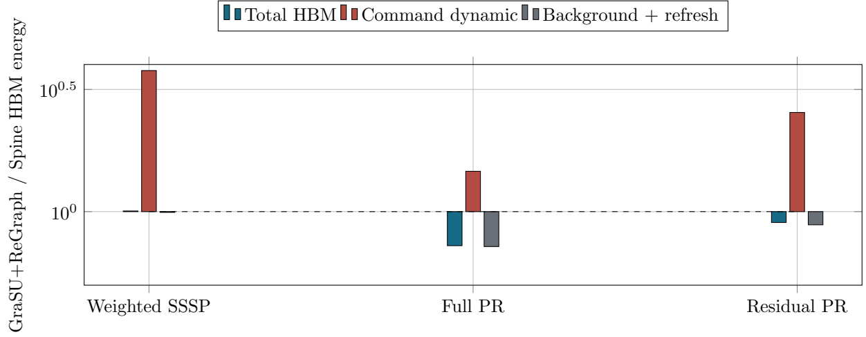
Figure 9: Matched all-32-controller DRAMSim3 energy on three compact holdout slices. The Spine SSSP values use exact per-controller subtraction of a reproduced quiescent cold prefix. Values above one mean GraSU+ReGraph uses more energy. This is HBM energy only, not total accelerator or board energy; asymmetric projected on-chip energy is intentionally excluded.
