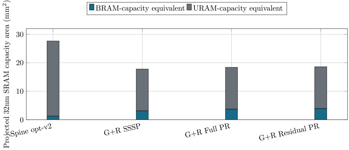
Figure 11: Conservative 32nm CACTI SRAM-capacity projection from routed BRAM and URAM allocations. It excludes logic, DSP, interconnect, clock, and I/O, so it is not a complete ASIC area estimate. Routed FPGA resources remain the primary implementation footprint in Table 2.
