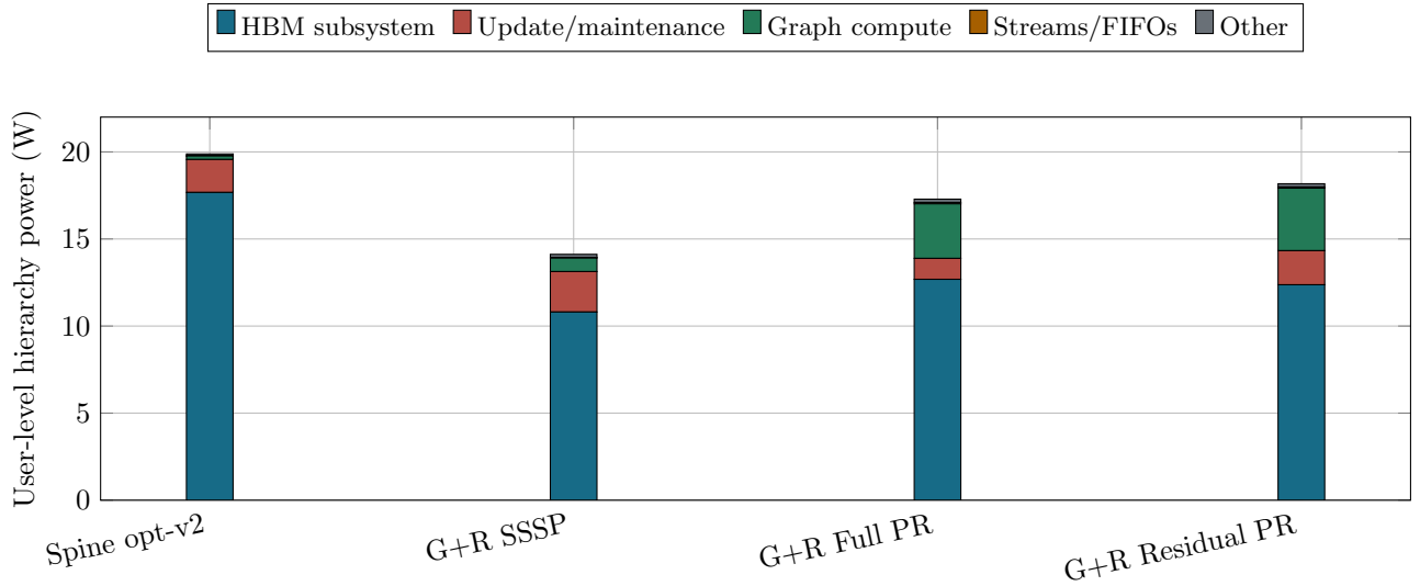
Figure 10: Vivado post-route vectorless power attribution at 150 MHz. Values are implementation-level component envelopes with Low confidence, not workload-calibrated energy. Platform residual and device static power are retained in the CSV ledger but excluded from the stacked user-logic bars.
