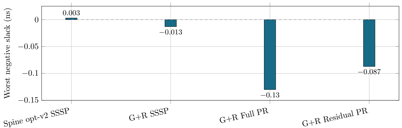
Figure 14: Post-route setup margin at the common 150 MHz target. Non-negative WNS closes timing; negative WNS identifies the remaining target miss.
