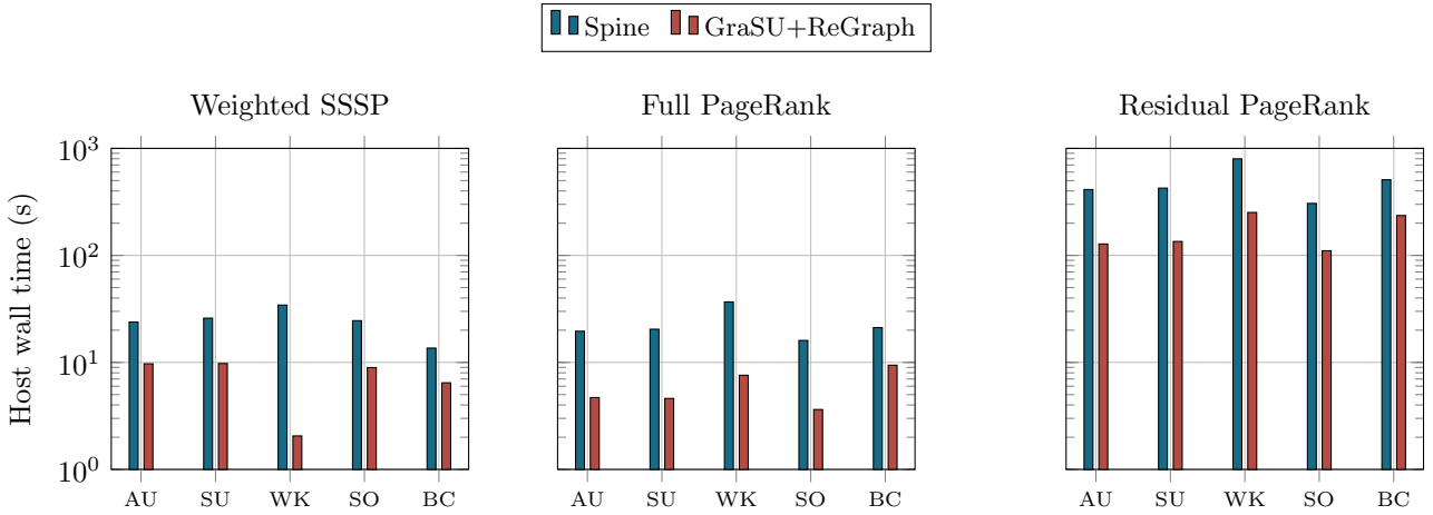
Figure 12: Observed simulator host runtime for the archived insertion-batch-8 runs. Every dataset has 8,192 base edges, while vertex counts vary from 2,004 to 10,326 as listed in Table 1. Each bar is one previously executed child-process observation from a parallel experiment matrix, not a repeated controlled benchmark. These values are engineering evidence for simulator-throughput planning and are not accelerator latency.
