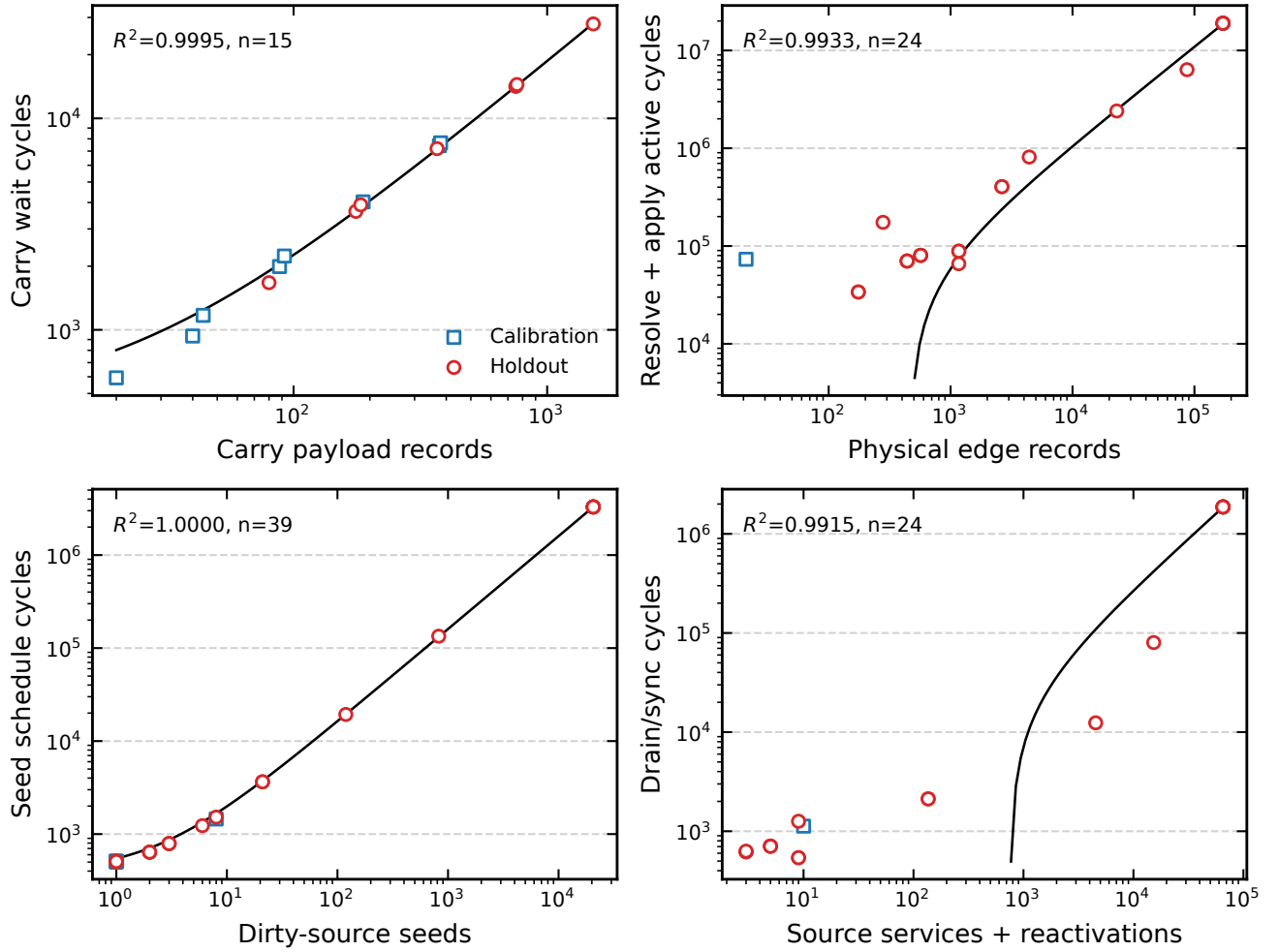
Figure 5: Direct execution counters versus mechanism-local cycles across 54 dual-oracle-admitted executions. Blue squares are calibration cases and red circles are holdout traces.
