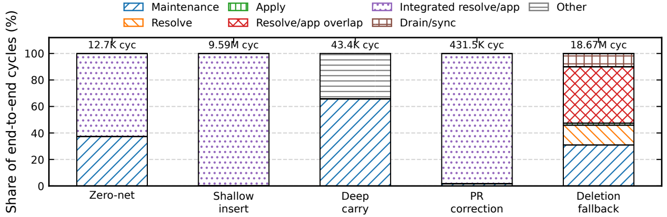
Figure 4: Exclusive, overlap-aware critical-path composition for zero-net, shallow insertion, deep carry, residual PageRank correction, and SSSP/CC nonmonotonic fallback. Absolute device cycles are printed above each bar.
