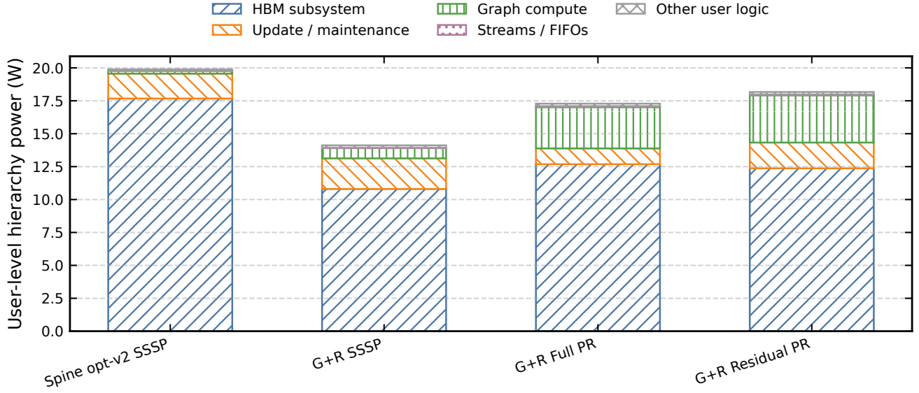
Figure 6: Vivado post-route vectorless hierarchy power at 150 MHz. The four bars are distinct routed builds; the Spine evidence covers SSSP only. Values use Vivado default activity with Low confidence and establish component attribution, not workload-calibrated energy or board power.
