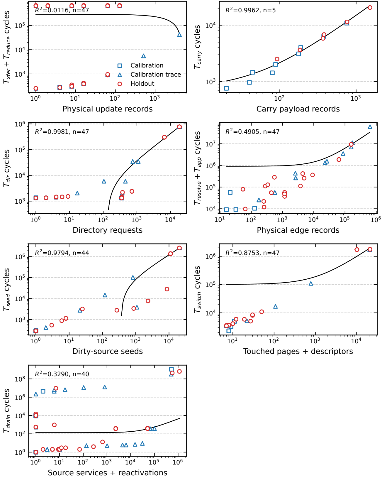
Figure 7: Direct execution counters versus mechanism-local cycles across 95 dual-oracle-admitted executions. Blue squares are calibration cases and red circles are holdout traces.
