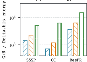
(b) HBM energy
