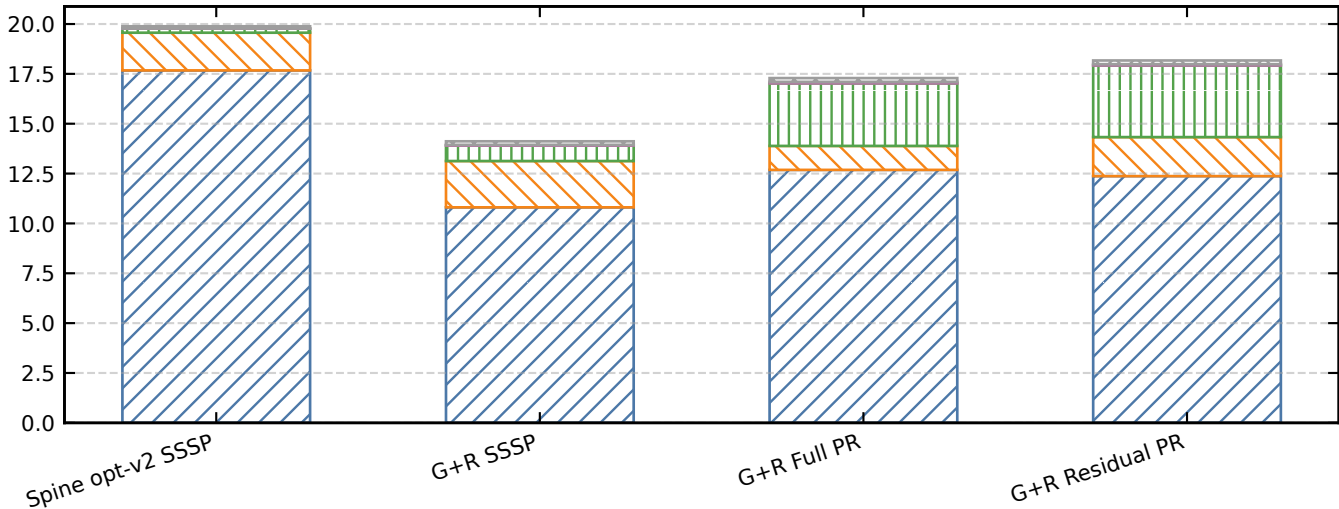
User-level hierarchy power (W)
