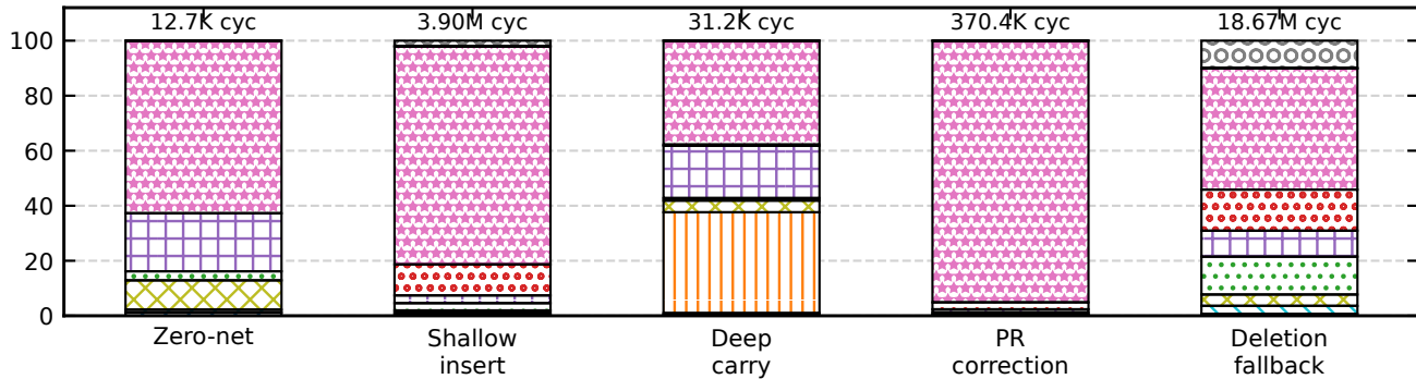
Share of end-to-end cycles (%)
