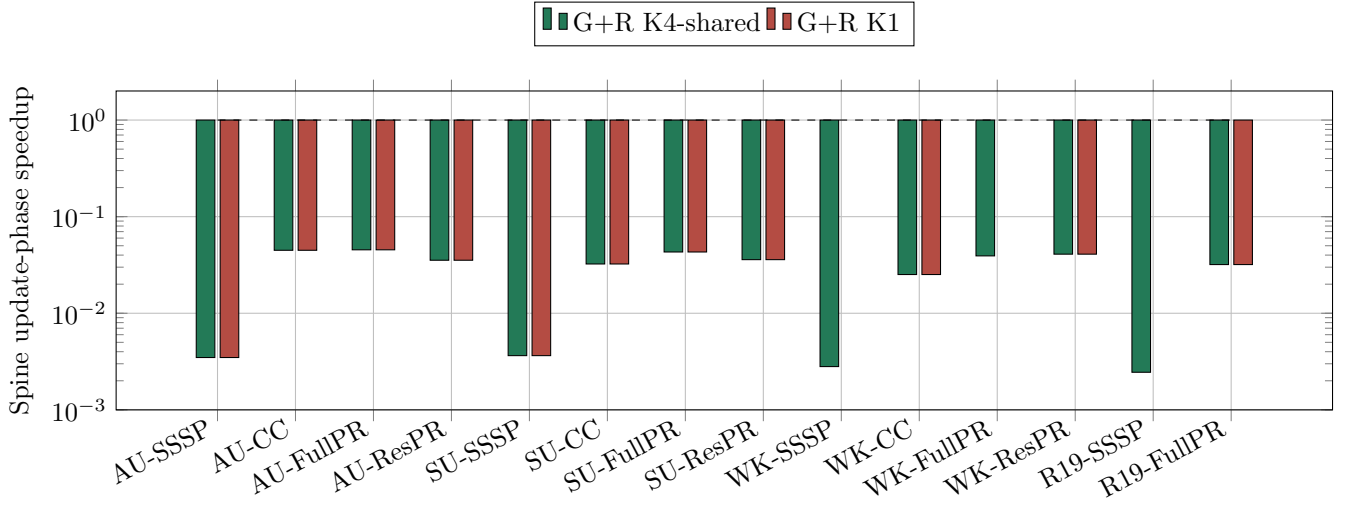
Figure 4: Update-phase cycles only. Values below one expose Spine’s current maintenance cost even when end-to-end execution favors Spine.
