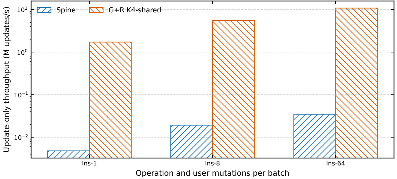
Figure 3: Correctness-gated AskUbuntu weighted-SSSP update-phase throughput. The current snapshot contains 3 of 9 planned operation–batch pairs. Ins uses the full materialized graph; Del and Wgt use the declared 64K-edge non-monotonic fallback slice. Missing points are not zeros.
