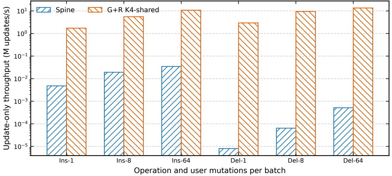
Figure 3: Correctness-gated AskUbuntu weighted-SSSP update-phase throughput. The current snapshot contains 6 of 9 planned operation–batch pairs. Ins uses the full materialized graph; Del and Wgt use the declared 64K-edge non-monotonic fallback slice. Missing points are not zeros.
