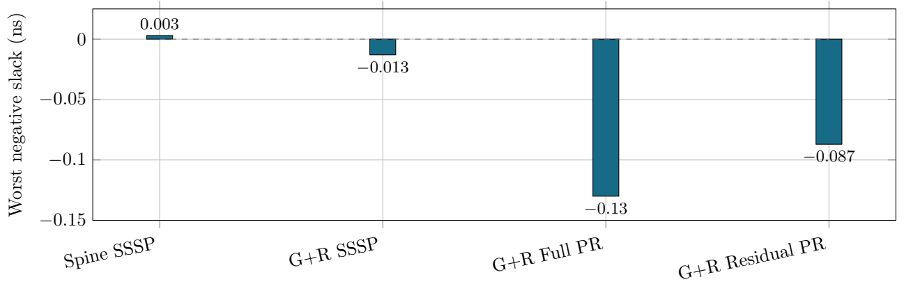
Figure 10: Post-route setup margin at each row’s stated target (152 MHz for Spine and 150 MHz for GraSU+ReGraph). Non-negative WNS closes timing; negative WNS identifies the remaining target miss.
