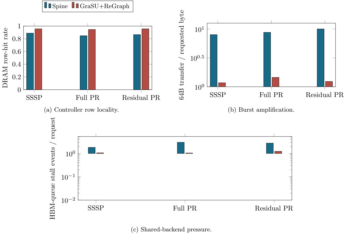
Figure 7: Phase-aligned physical HBM behavior for batch-8 insertion on five compact real-topology slices. The DRAM-Sim3 command ledger equals accepted AXI requests on every row. Stall values count rejected port attempts, so multiple events may occur in one cycle. Spine weighted SSSP uses an exact quiescent cold-prefix subtraction to align its controller window.
